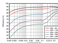
Efficiency versus Output Current V_{OUT} = 5V , 400kHz
