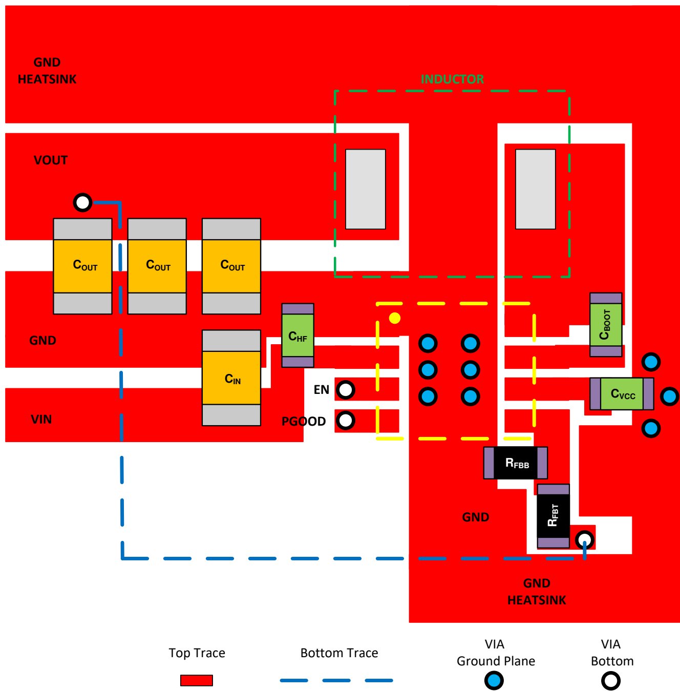
Figure 8-24. Example Layout
