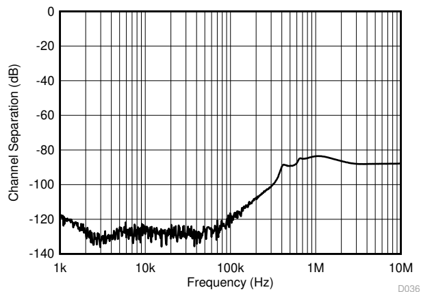
Figure 5-31. Channel Separation
