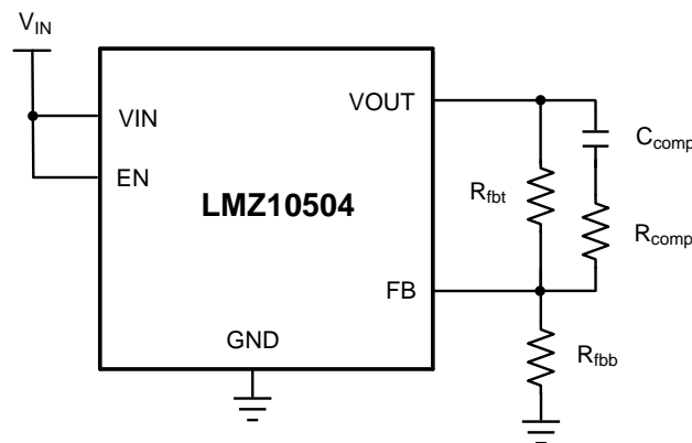
Figure 22. Loop Compensation Control Components
