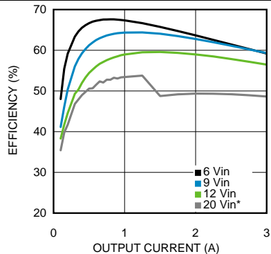
Figure 33. Efficiency 1-V Output at 85°C Ambient
