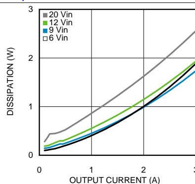
Figure 26. Dissipation 2.5-V Output at 85°C Ambient
