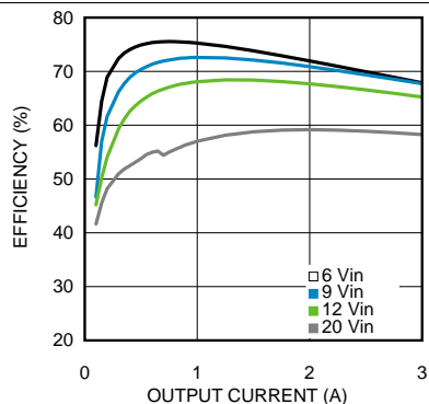
Figure 31. Efficiency 1.2-V Output at 85°C Ambient
