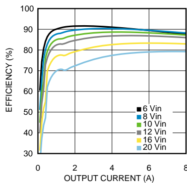
Figure 3. Efficiency 3.3-V Output at 25°C
