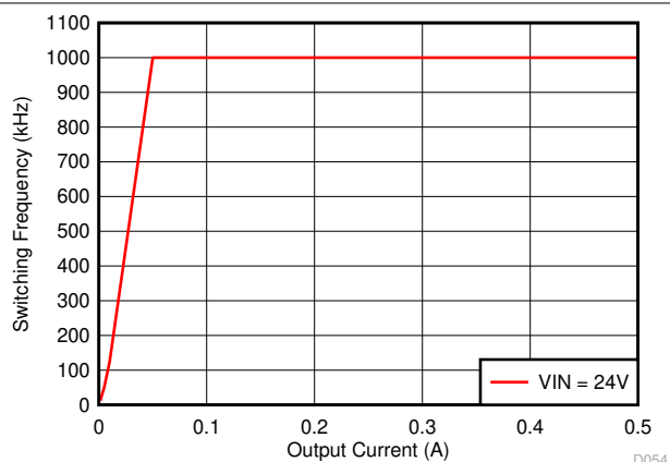
Figure 7-27. Auto PFM Mode Switching Frequency vs Output Current
