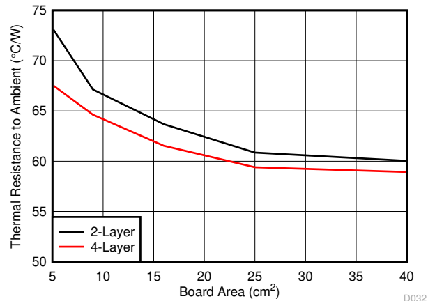
Figure 7-8. Package Thermal Resistance vs Board Copper Area, No Air Flow
