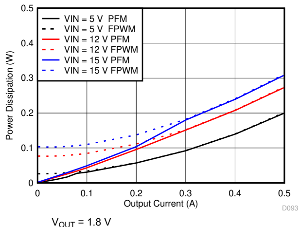
Figure 7-14. Power Dissipation
