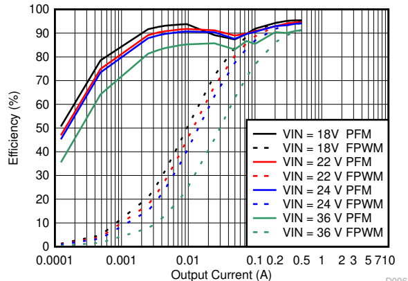
Figure 9-24. Efficiency
