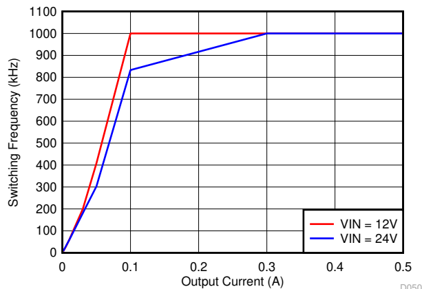
Figure 7-26. Auto PFM Mode Switching Frequency vs Output Current
