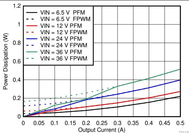
Figure 7-9. Power Dissipation
