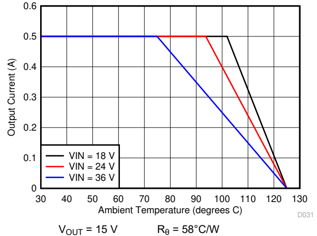
Figure 7-22. Ambient Temperature vs Output Current
