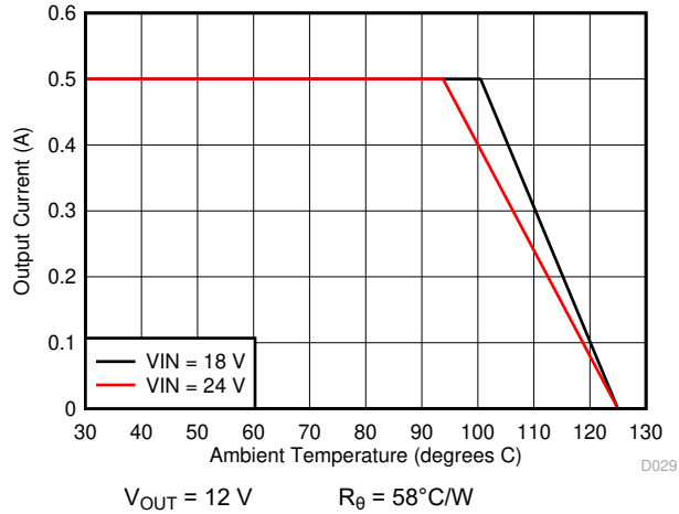
Figure 7-21. Ambient Temperature vs Output Current
