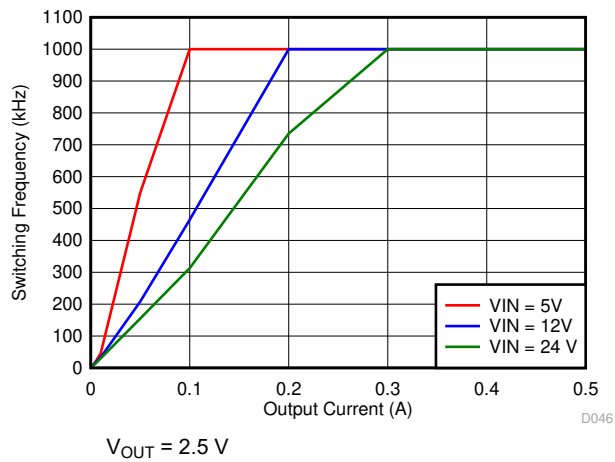
Figure 7-23. Auto PFM Mode Switching Frequency vs Output Current
