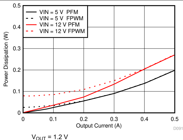
Figure 7-15. Power Dissipation
