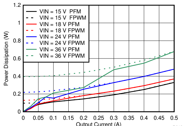
Figure 7-10. Power Dissipation
