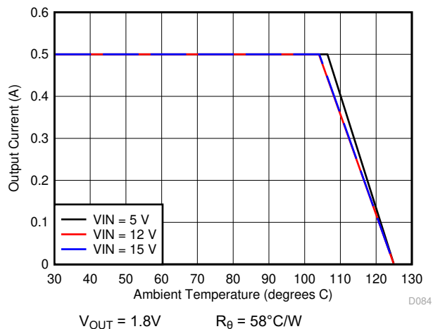
Figure 7-17. Ambient Temperature vs Output Current
