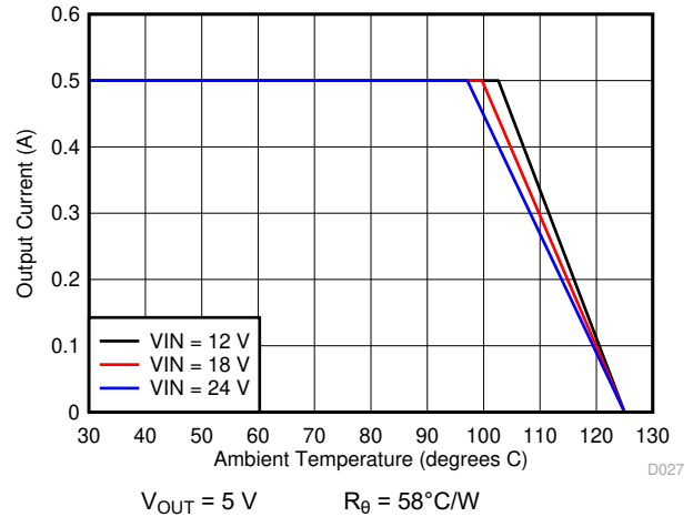
Figure 7-20. Ambient Temperature vs Output Current
