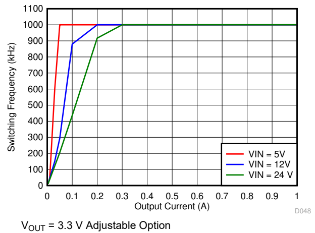
Figure 7-24. Auto PFM Mode Switching Frequency vs Output Current
