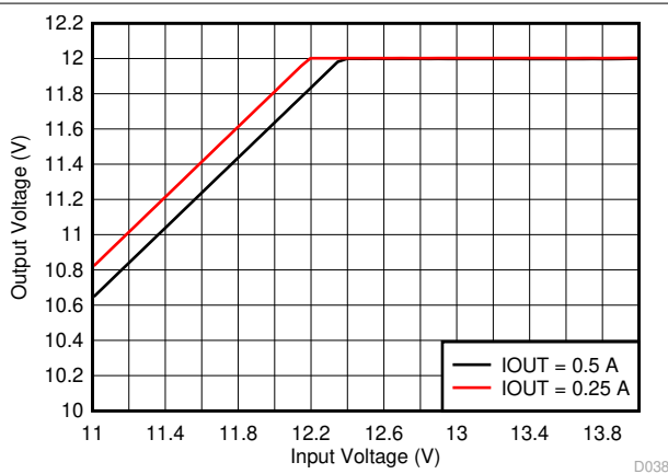
Figure 7-3. Dropout Voltage
