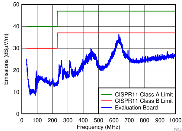
Figure 7-7. Radiated EMI
