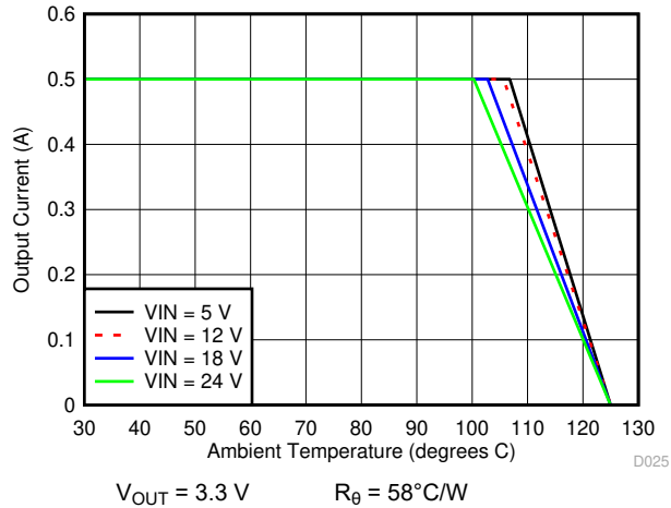
Figure 7-19. Ambient Temperature vs Output Current
