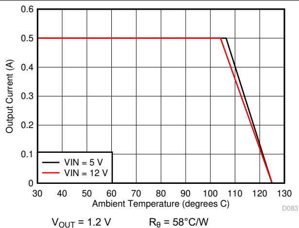
Figure 7-16. Ambient Temperature vs Output Current
