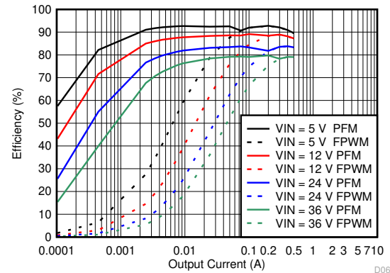
Figure 9-43. Efficiency for V_{OUT} = 3.3\text{ V}
