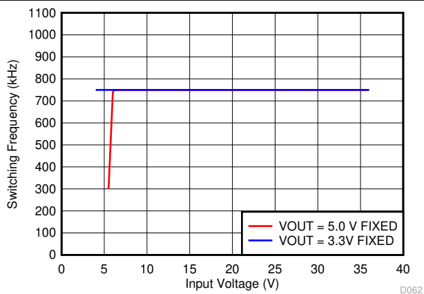
Figure 7-31. Switching Frequency vs Input Voltage for Fixed Output Options at Full Load
