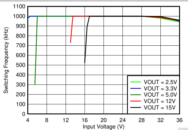
Figure 7-30. Switching Frequency vs Input Voltage for Adjustable Output Options at Full Load
