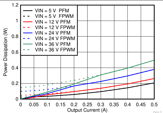
Figure 7-10. Power Dissipation
