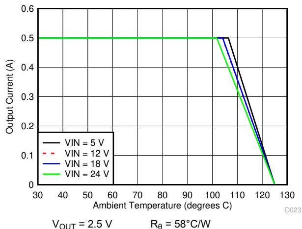
Figure 7-18. Ambient Temperature vs Output Current
