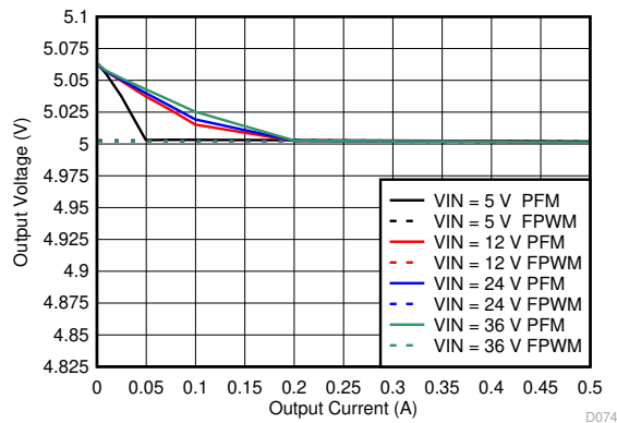
Figure 9-44. Line and Load Regulation for V_{OUT} = 5\text{ V}
