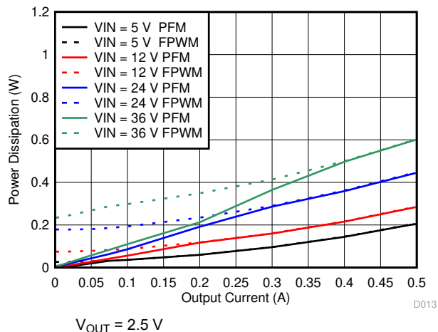
Figure 7-13. Power Dissipation
