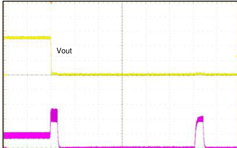
Figure 8-2. Hiccup Operation
