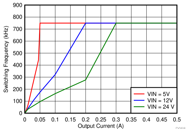
Figure 7-25. Auto PFM Mode Switching Frequency vs Output Current
