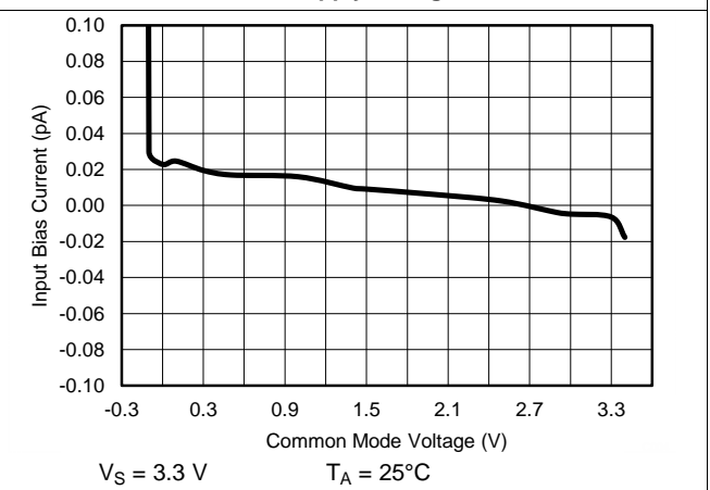
Figure 18. Input Bias Current vs Common Mode Voltage at 3.3 V
