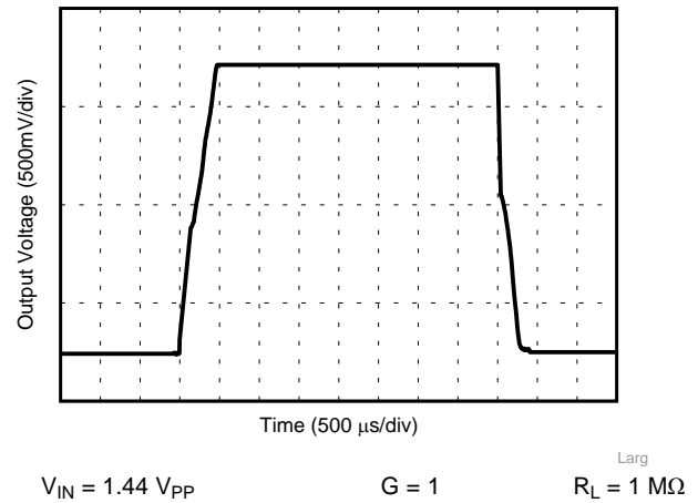
Figure 34. Large-Signal Response, 1.8V
