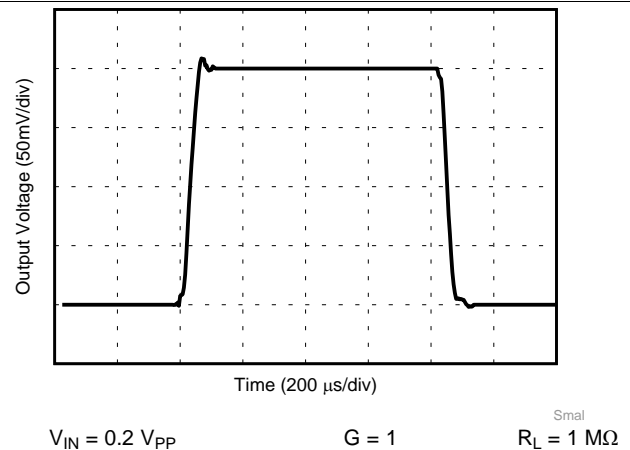
Figure 36. Small-Signal Response, 1.8V
