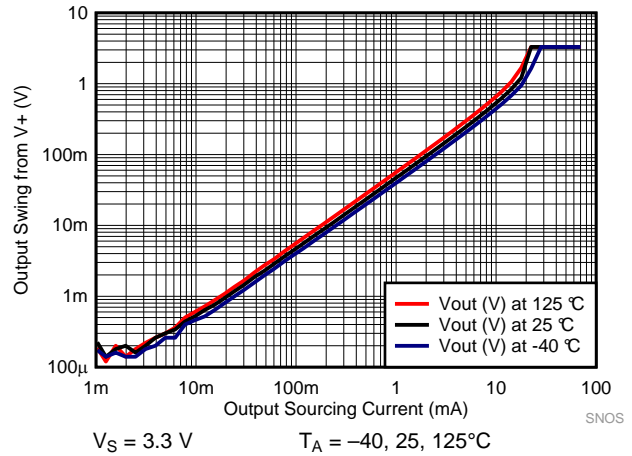
Figure 32. Output Swing vs Sourcing Current, 3.3 V
