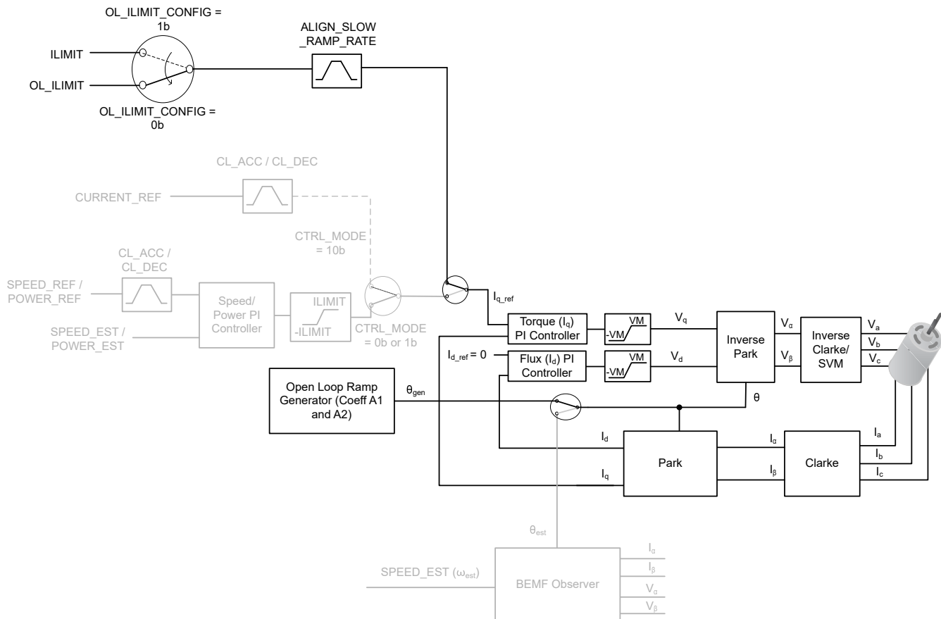
Figure 7-24. Open Loop
