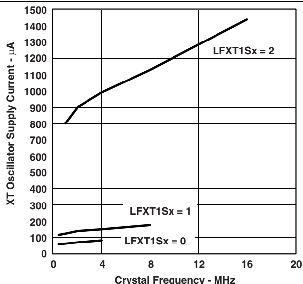
Figure 4-25. XT Oscillator Supply Current vs Crystal Frequency, C_{L,eff} = 15\text{ pF} , T_A = 25^\circ\text{C}
