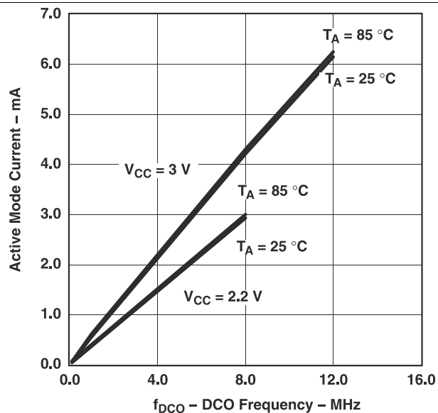
Figure 4-4. Active-Mode Current vs DCO Frequency
