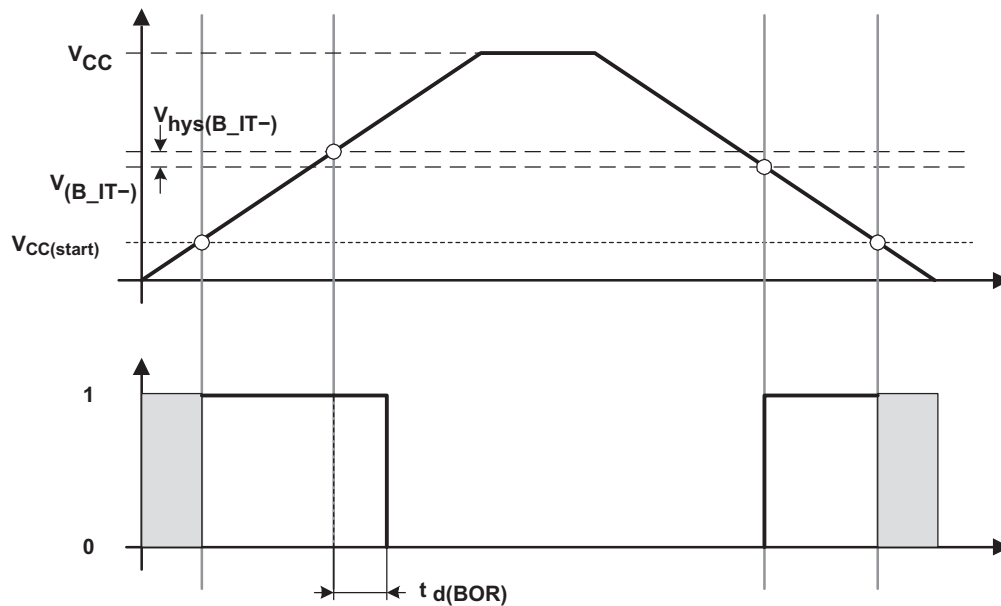
Figure 4-10. POR/Brownout Reset (BOR) vs Supply Voltage
