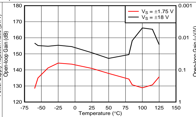
Figure 38. Open-Loop Gain vs Temperature
