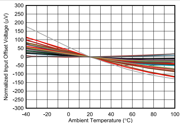
Figure 6-21. Typical Input Offset Voltage Over Temperature
