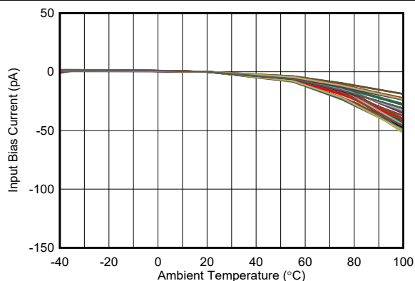
Figure 6-23. Typical Input Bias Current Over Temperature
