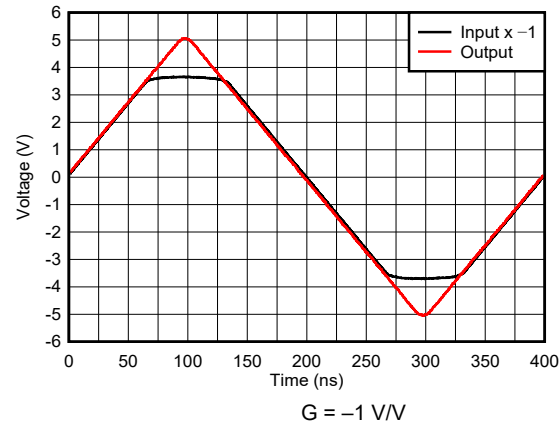
Figure 6-27. Inverting Overdrive Recovery
