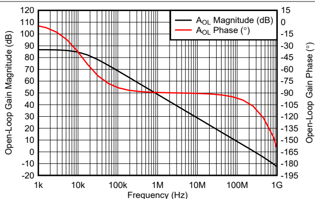
Figure 6-19. Open-Loop Gain and Phase
