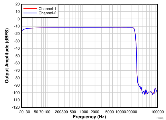
Figure 7-16. PCM1821-Q1: Frequency Response With a -12\text{-dB} Input
