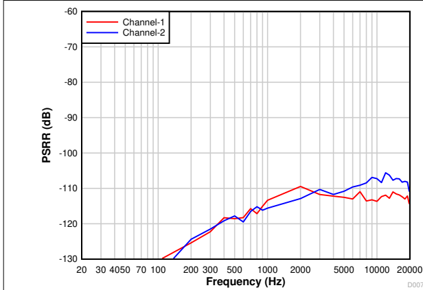
Figure 7-7. PCM1820-Q1: Power-Supply Rejection Ratio vs Ripple Frequency With a 100-mV pp Amplitude
