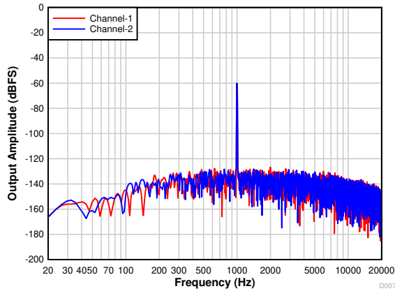
Figure 7-19. PCM1821-Q1: FFT With a -60-dBr Input and DRE Enabled
