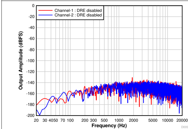
Figure 7-9. PCM1820-Q1: FFT With Idle Input and DRE Disabled
