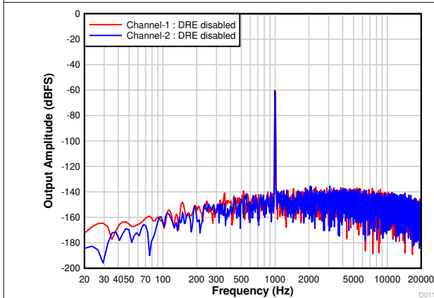
Figure 7-11. PCM1820-Q1: FFT With a -60-dBr Input and DRE Disabled
