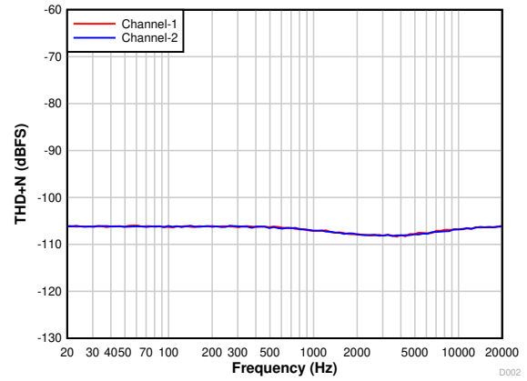
Figure 7-14. PCM1821-Q1: THD+N vs Input Frequency With a -60\text{-dB} Input
