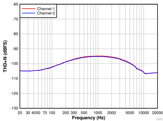
Figure 7-15. PCM1821-Q1: THD+N vs Input Frequency With a -1\text{-dB} Input
