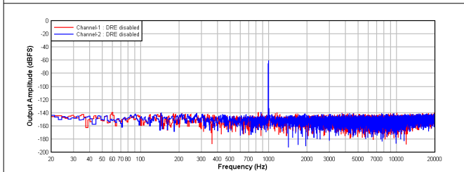
Figure 9-4. PCM1820-Q1: FFT With a –60-dBr Input With DRE Disabled
