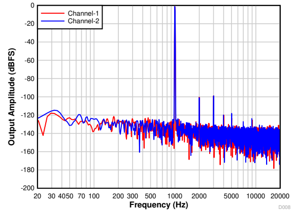
Figure 7-20. PCM1821-Q1: FFT With a -1-dBr Input
