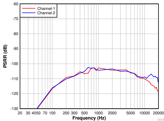
Figure 7-17. PCM1821-Q1: Power-Supply Rejection Ratio vs Ripple Frequency With a 100\text{-mV}_{PP} Amplitude
