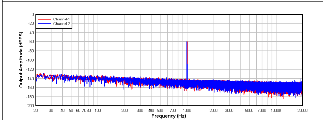
Figure 9-6. PCM1821-Q1: FFT With a –60-dBr Input
