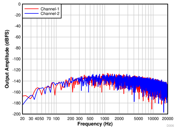
Figure 7-18. PCM1821-Q1: FFT With Idle Input and DRE Disabled
