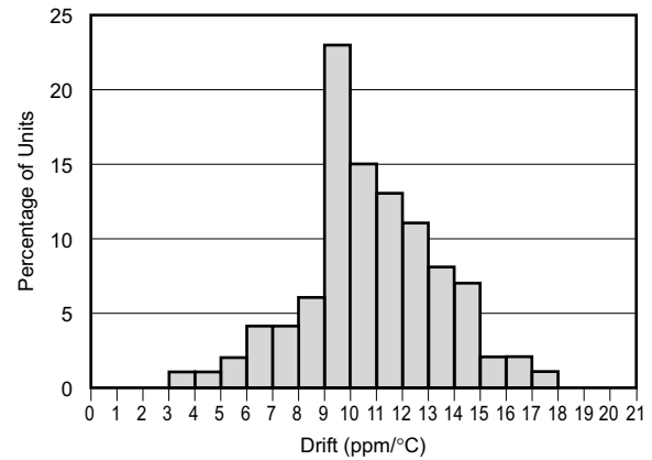
Figure 6-2. Temperature Drift ( -40^\circ\text{C} to +125^\circ\text{C} )
