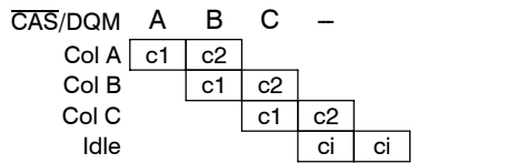
Nonpipelined 1-cycle/column EDO (CT = 0001) reads, read transfers, split read transfers
