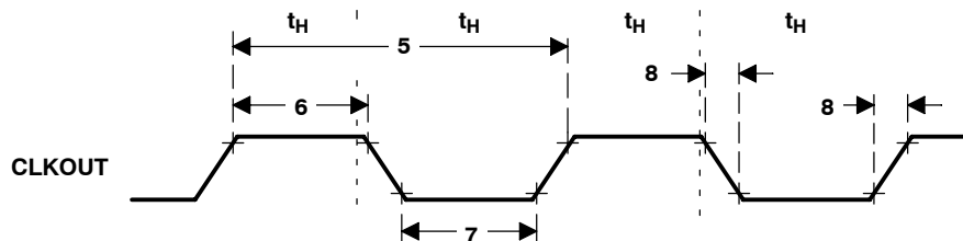
Figure 109. CLKOUT Timing
