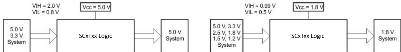
Figure 6-2. SCxT Up and Down Translation Example
