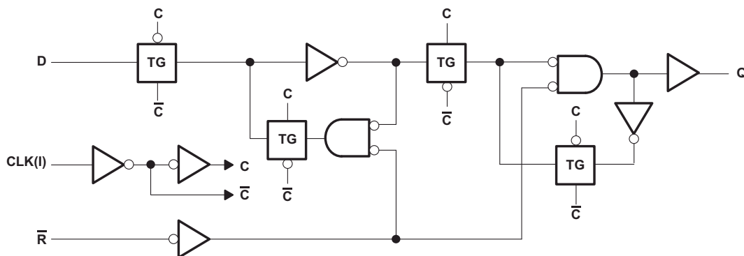
Simplified Schematic
