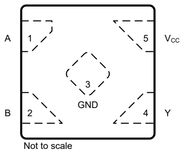
Figure 4-1. DTX Package, 5-Pin X2SON (Top View)
