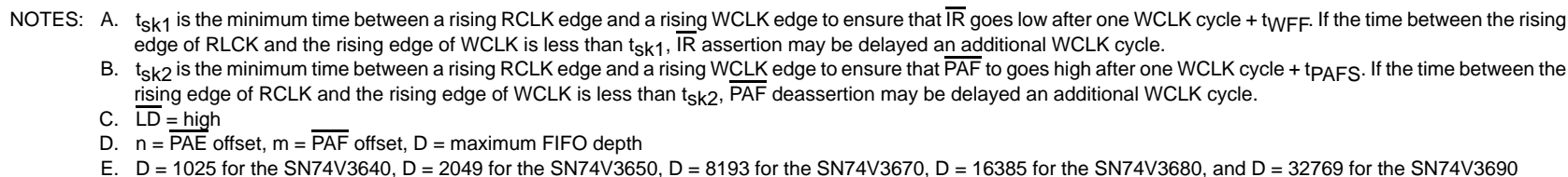
Figure 7. Read Timing (FWFT Mode)
