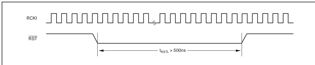
Figure 3. Reset Pulswidth Requirement
