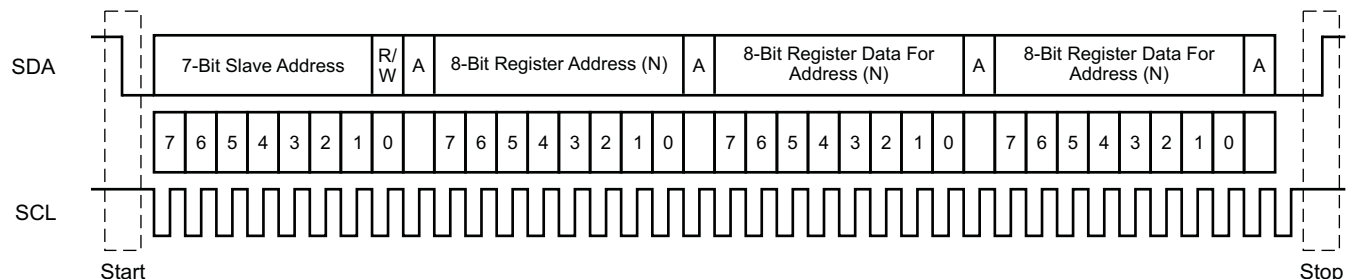
Figure 46. Typical I 2 C Sequence
