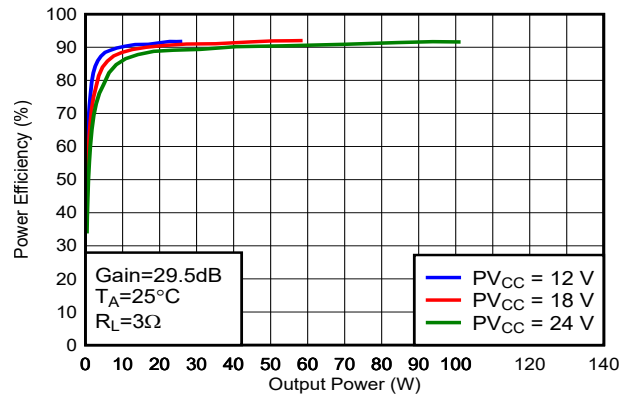
1SPW Modulation F SW =384kHz Load = 3Ω PBTTL Mode Gain=29.5dB T A =25°C R L =3Ω Figure 5-77. Efficiency vs Output Power
