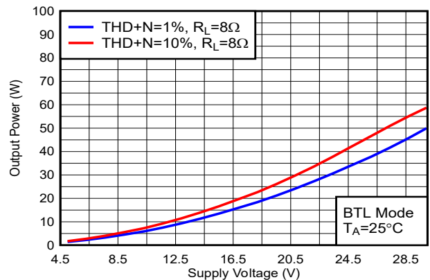
Figure 5-14. Output Power vs Supply Voltage
