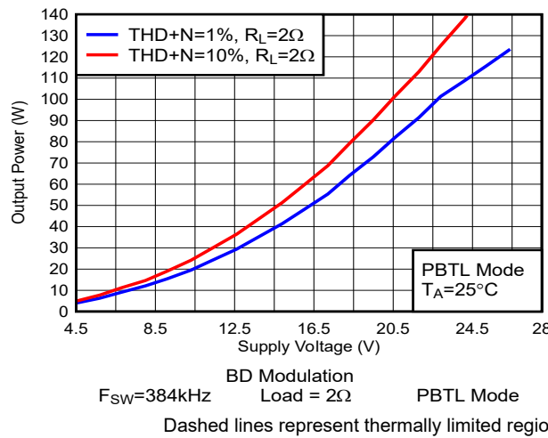
Figure 5-54. Output Power vs Supply Voltage
