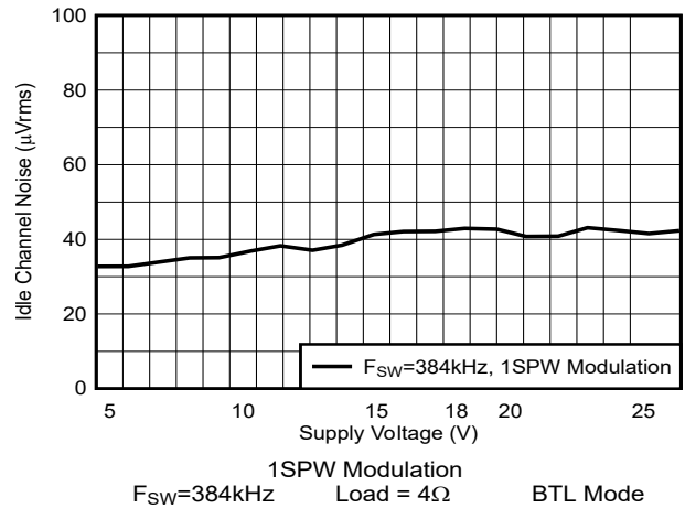
Figure 5-38. Idle Channel Noise vs Supply Voltage
