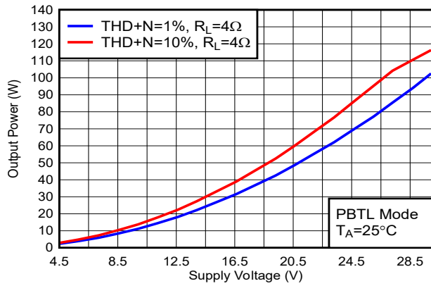
BD Modulation F SW =384kHz Load = 4Ω PBTLM Mode Figure 5-56. Output Power vs Supply Voltage
