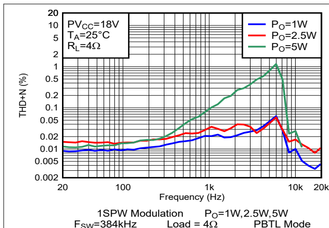
Figure 5-66. THD+N vs Frequency-PBTL
