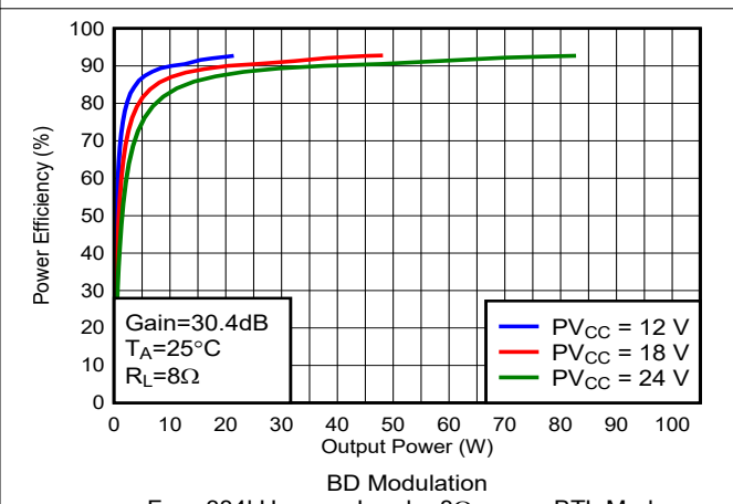
Figure 5-24. Efficiency vs Output Power
