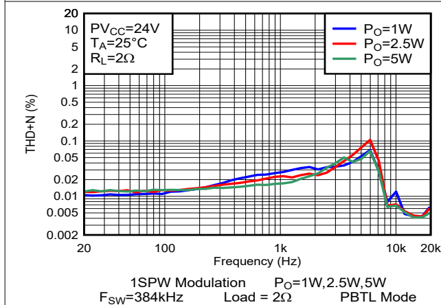
Figure 5-64. THD+N vs Frequency-PBTL
