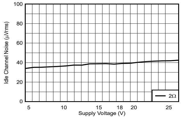
BD Modulation F SW =384kHz Load = 2Ω PBTLM Mode Figure 5-57. Idle Channel Noise vs Supply Voltage
