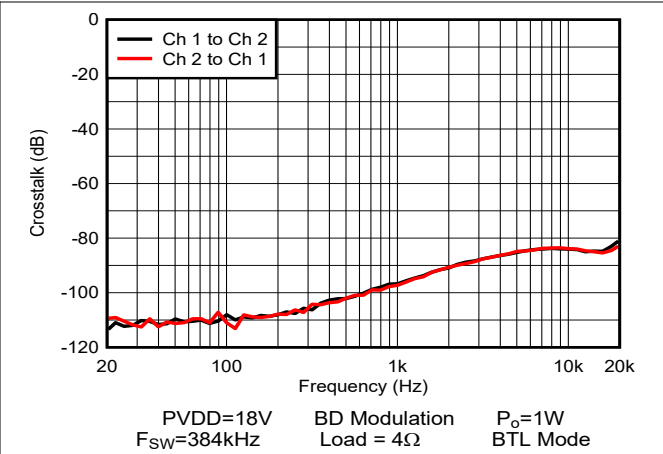
Figure 5-20. Crosstalk
