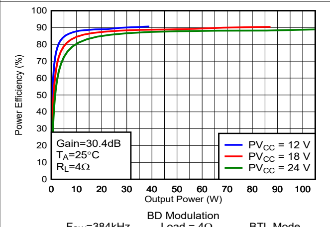
Figure 5-22. Efficiency vs Output Power
