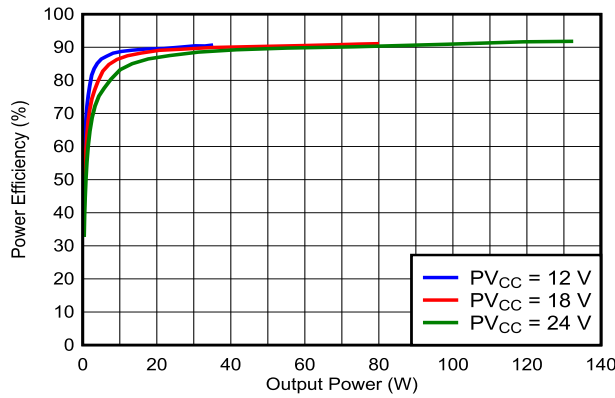
1SPW Modulation F SW =384kHz Load = 2Ω PBTTL Mode Figure 5-76. Efficiency vs Output Power
