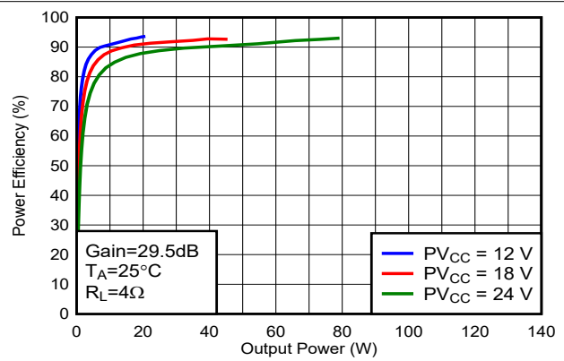
BD Modulation F SW =384kHz Load = 4Ω PBTLM Mode Figure 5-61. Efficiency vs Output Power
