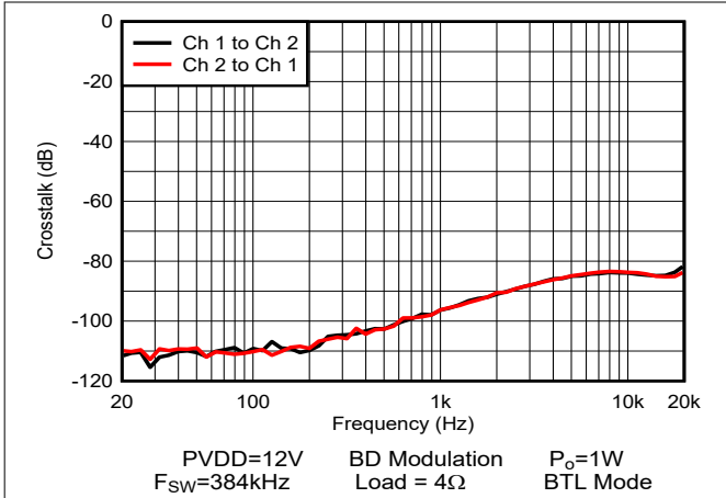
Figure 5-19. Crosstalk
