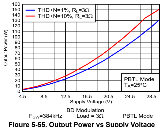
Figure 5-55. Output Power vs Supply Voltage
