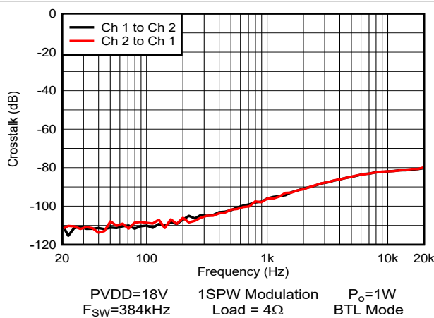
Figure 5-41. Crosstalk
