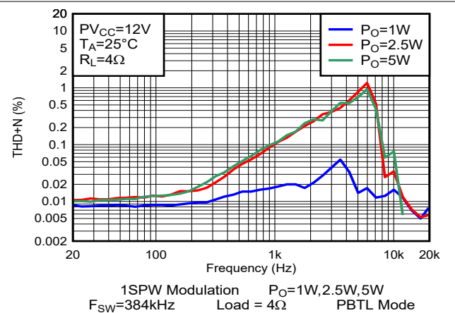
Figure 5-65. THD+N vs Frequency-PBTL
