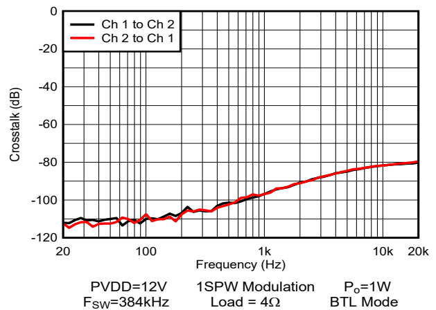
Figure 5-40. Crosstalk
