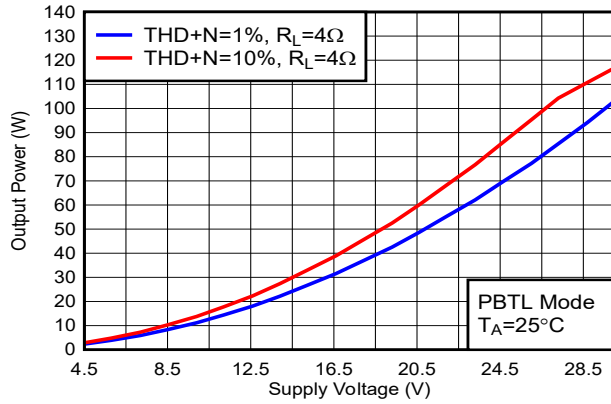
1SPW Modulation F SW =384kHz Load = 4Ω PBTTL Mode Figure 5-74. Output Power vs Supply Voltage
