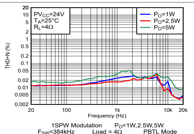
Figure 5-67. THD+N vs Frequency-PBTL
