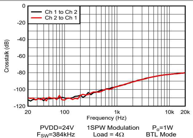
Figure 5-42. Crosstalk
