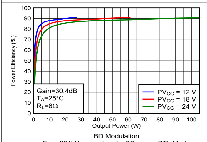
Figure 5-23. Efficiency vs Output Power
