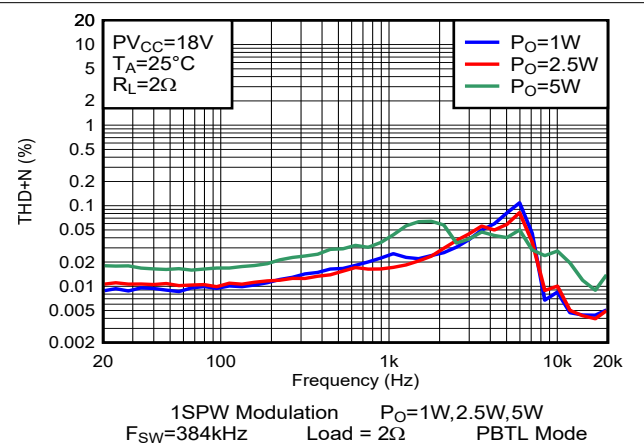
Figure 5-63. THD+N vs Frequency-PBTL
