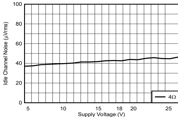
BD Modulation F SW =384kHz Load = 4Ω PBTLM Mode Figure 5-58. Idle Channel Noise vs Supply Voltage
