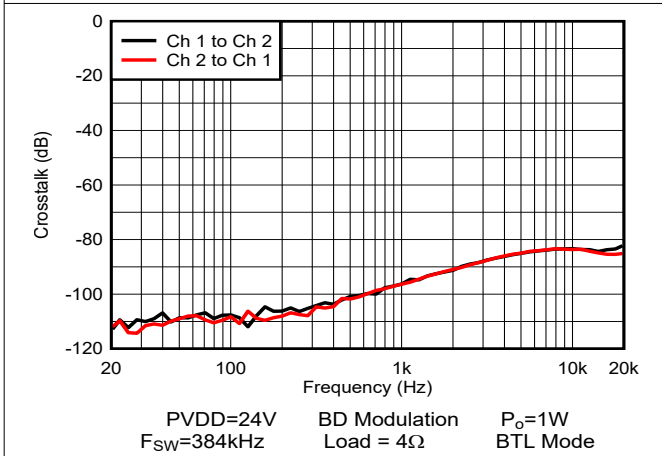
Figure 5-21. Crosstalk
