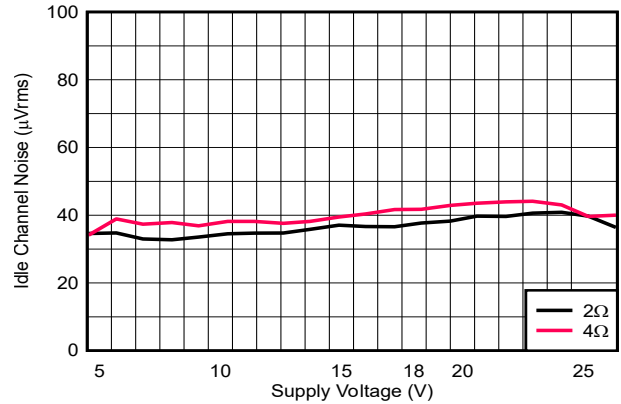
1SPW Modulation F SW =384kHz Load = 2Ω, 4Ω PBTTL Mode Figure 5-75. Idle Channel Noise vs Supply Voltage
