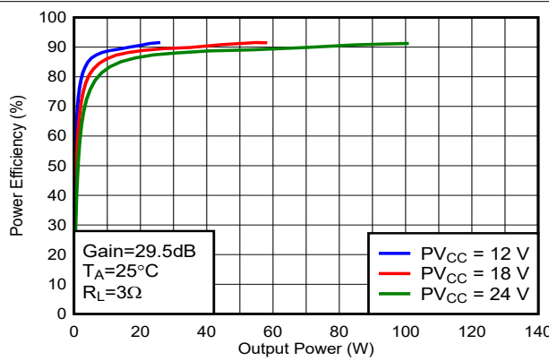
BD Modulation F SW =384kHz Load = 3Ω PBTLM Mode Figure 5-60. Efficiency vs Output Power
