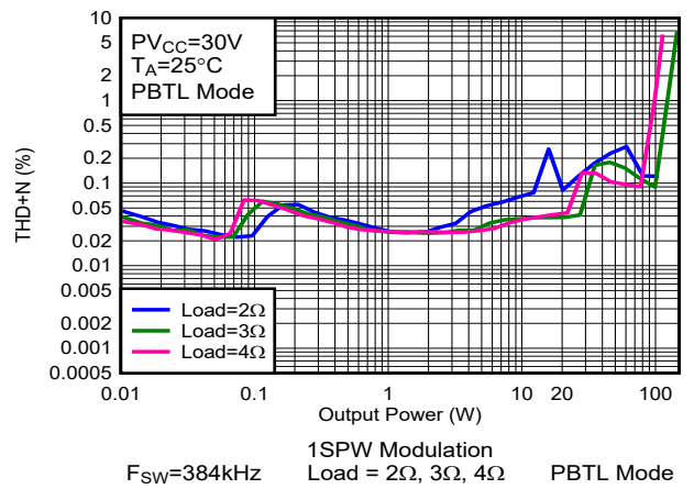
Figure 5-53. THD+N vs Power-PBTL
