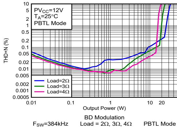
Figure 5-50. THD+N vs Output Power-PBTL
