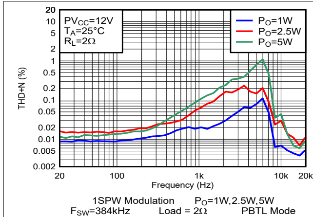
Figure 5-62. THD+N vs Frequency-PBTL
