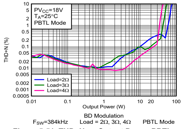
Figure 5-51. THD+N vs Output Power-PBTL
