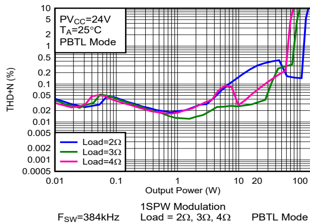
Figure 5-52. THD+N vs Output Power-PBTL
