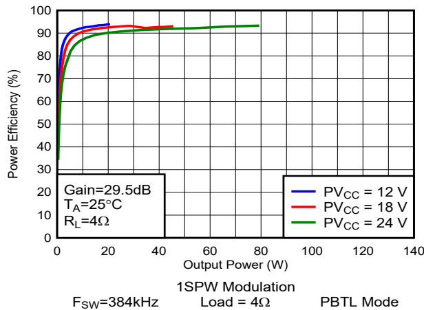
1SPW Modulation F SW =384kHz Load = 4Ω PBTTL Mode Gain=29.5dB T A =25°C R L =4Ω Figure 5-78. Efficiency vs Output Power
