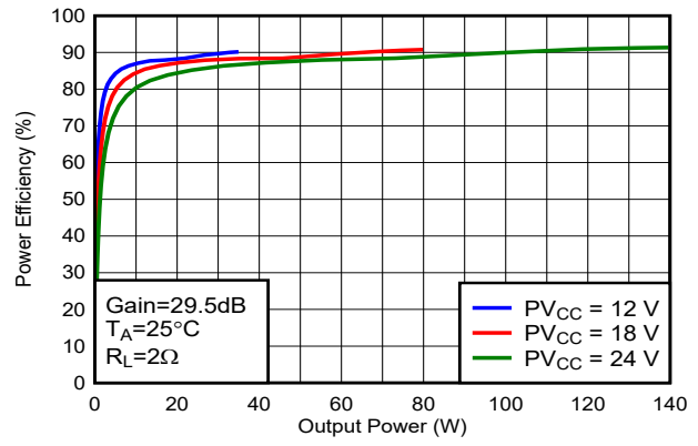
BD Modulation F SW =384kHz Load = 2Ω PBTLM Mode Figure 5-59. Efficiency vs Output Power
