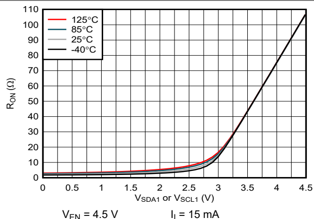
Figure 5-2. On-Resistance ( R_{ON} ) vs Input Voltage ( V_{SDA1} or V_{SCL1} )
