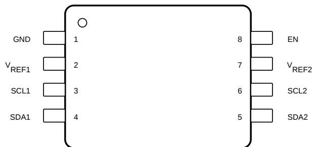
Figure 4-1. DCU Package, 8-Pin VSSOP, Top View
