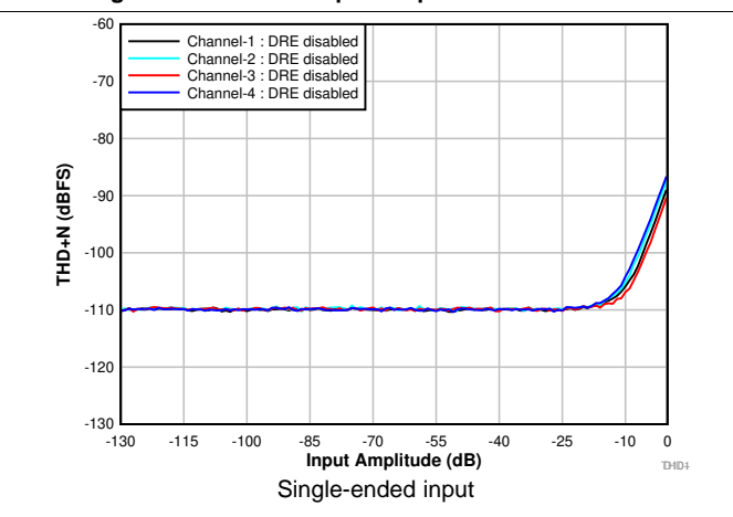
Figure 8. THD+N vs Input Amplitude With DRE Disabled
