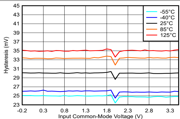
Figure 5-8. Hysteresis vs. Common-Mode, 3.3V
