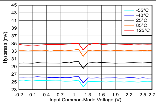
Figure 5-6. Hysteresis vs. Common-Mode, 2.5V
