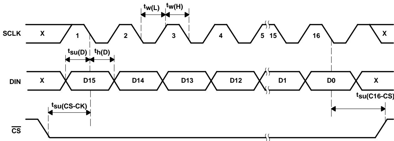
Figure 1. Timing Diagram
