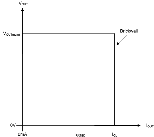
Figure 7-1. Current Limit
