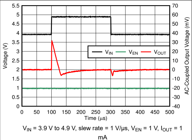
Figure 5-18. Line Transient
