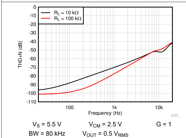
Figure 6-23. THD + N vs Frequency
