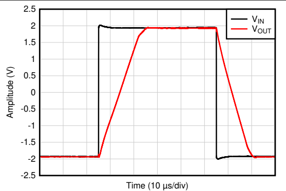
Figure 6-33. Overload Recovery
