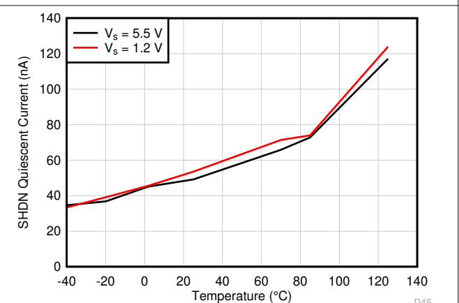
Figure 6-42. Shutdown Mode Quiescent Current vs Temperature
