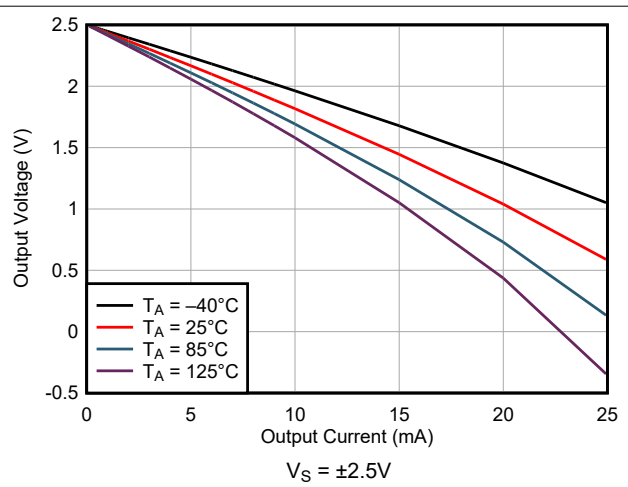
Figure 5-24. Output Voltage Swing vs Output Current (Sourcing)
