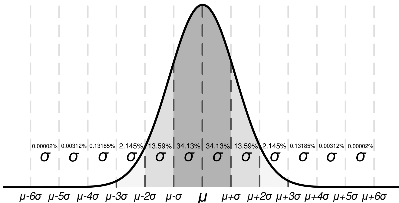
Figure 6-7. Gaussian Distribution
