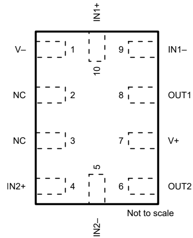
Figure 4-5. TLV9142 RUG Package, 10-Pin X2QFN (Top View)
