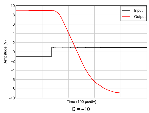
Figure 5-36. Overload Recovery (Positive)
