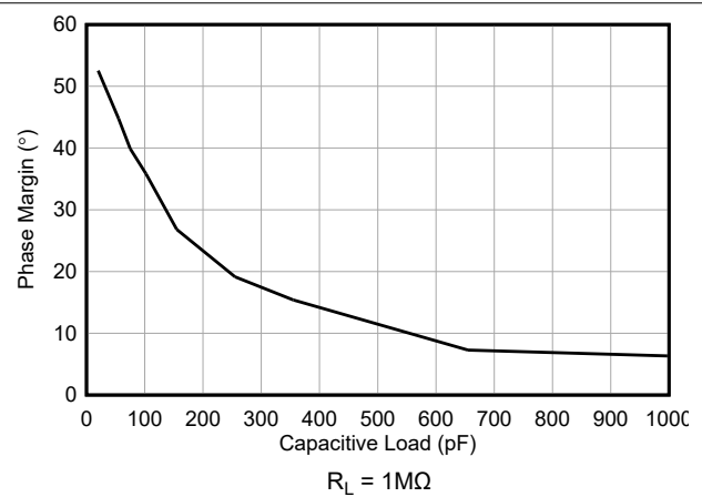
Figure 5-4. Phase Margin vs Capacitive Load
