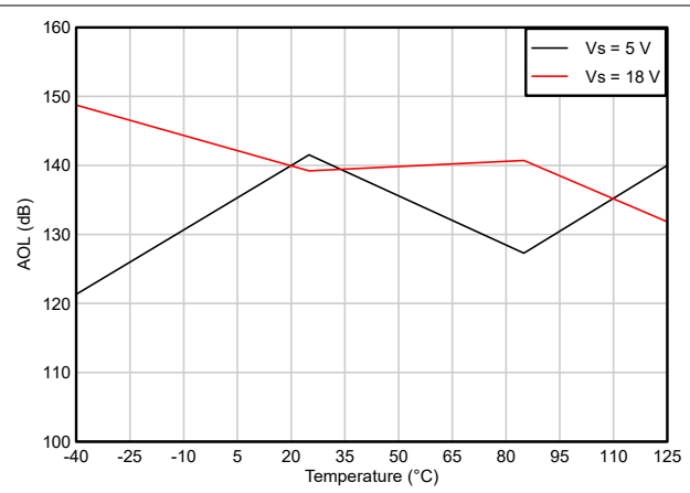
Figure 5-32. Open-Loop Gain vs Temperature
