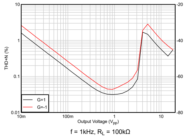
Figure 5-10. THD+N vs Output Voltage
