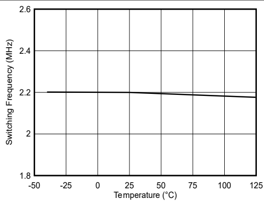
Figure 5-5. f_{SW} 2.2MHz
