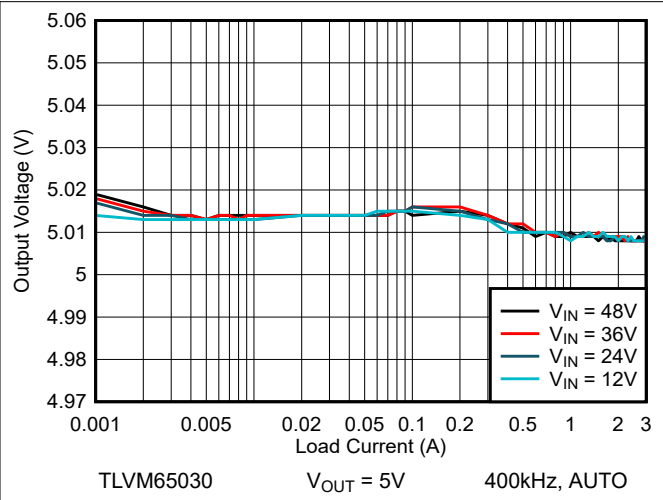
Figure 7-5. Line and Load Regulation
