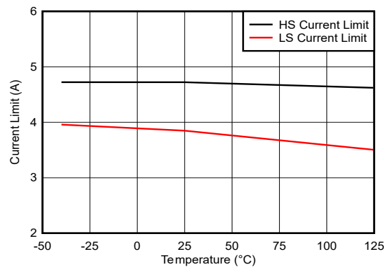
Figure 5-8. Current Limit
