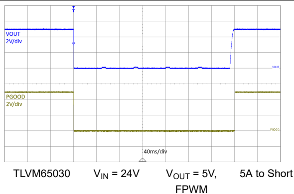
Figure 7-12. Short Circuit Applied
