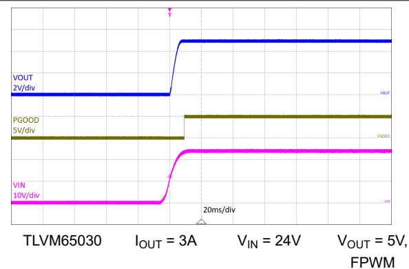
Figure 7-15. Start-Up
