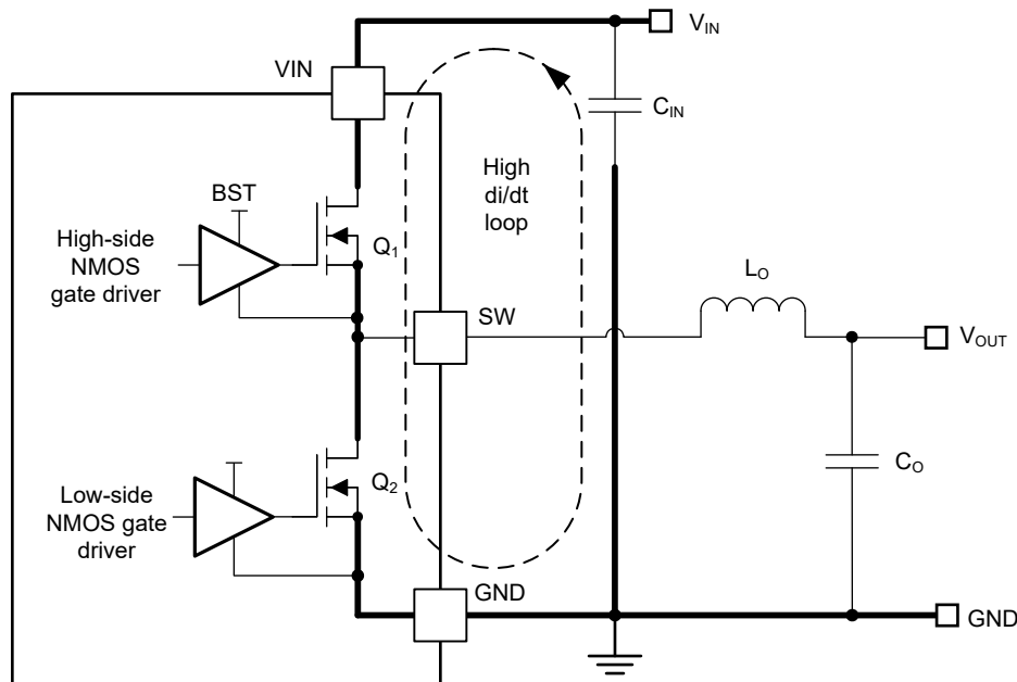
Figure 7-18. Current Loops With Fast Edges
