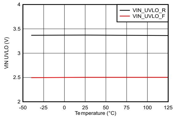
Figure 5-3. Enable UVLO
