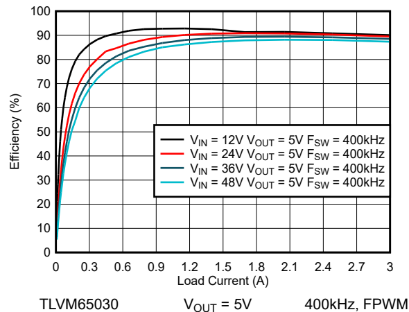
Figure 7-10. Efficiency
