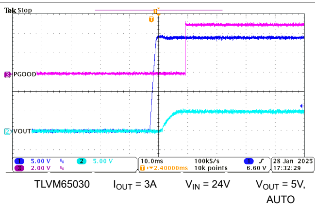
Figure 7-8. Start-Up
