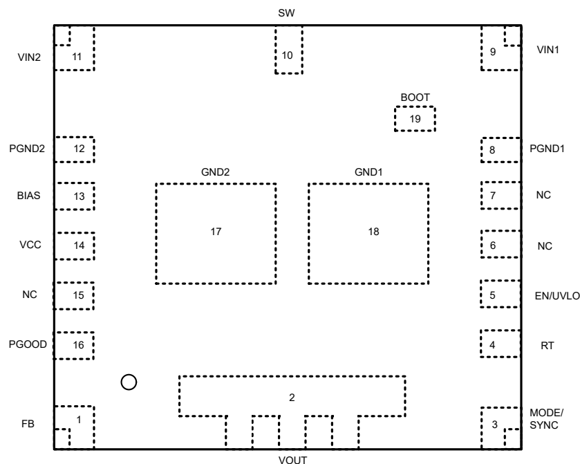
Figure 4-1. 19-Pin VCG, QFN-FCMOD Package (Top View)
