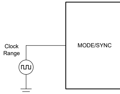
Figure 6-3. Typical Implementation Allowing Synchronization Using the MODE/SYNC Pin
