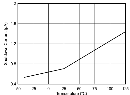
Figure 5-2. Shutdown Input Current
