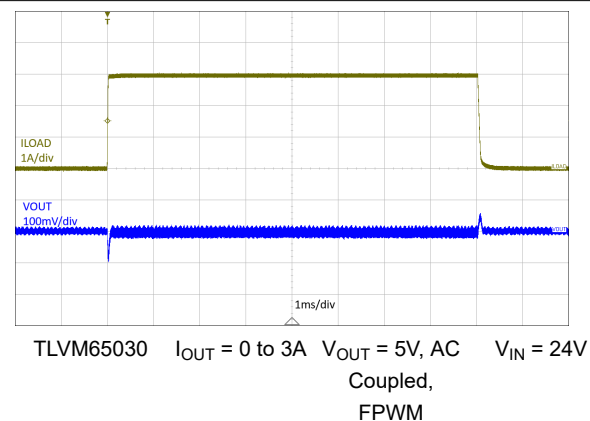
Figure 7-13. Load Transient (0 to 100%)
