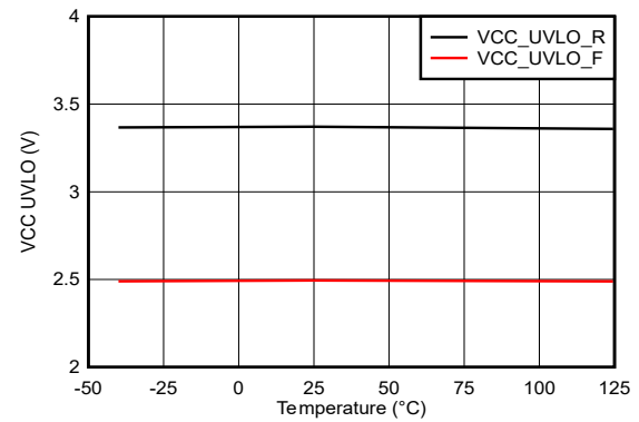
Figure 5-4. VCC UVLO
