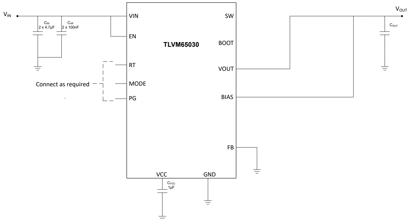
Figure 7-1. Example Application Circuit for Fixed Output Voltage Mode With TLVM65030
