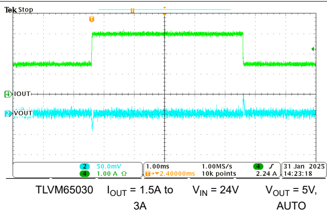
Figure 7-6. Load Transient (50% to 100%)
