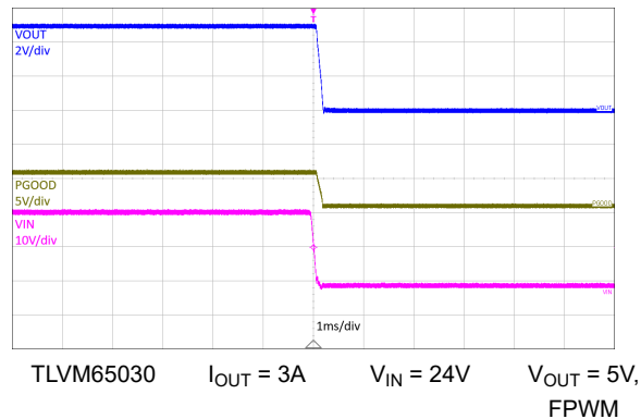
Figure 7-16. Shutdown
