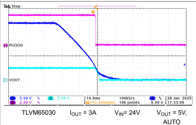
Figure 7-9. Shutdown
