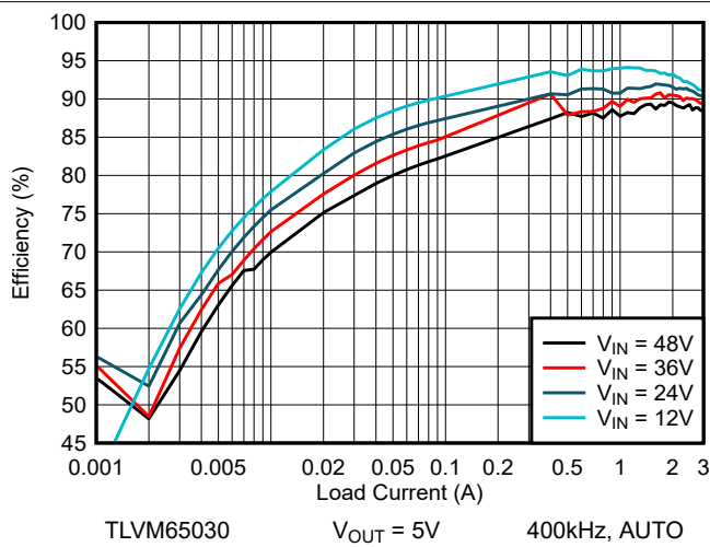
Figure 7-4. Efficiency
