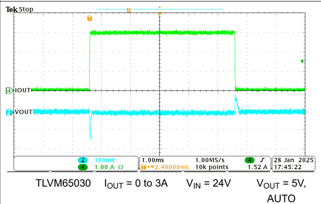
Figure 7-7. Load Transient (0% to 100%)
