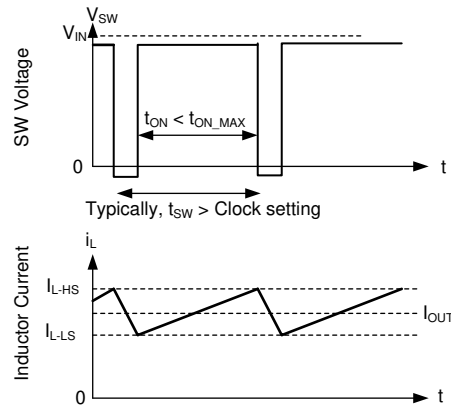
Figure 6-8. Current Limit Waveforms
