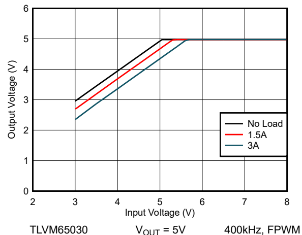
Figure 7-11. Dropout
