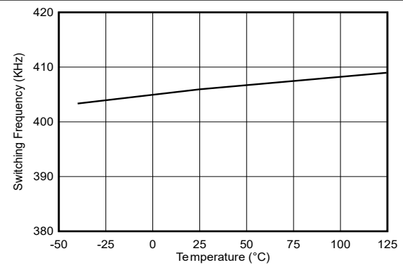
Figure 5-6. f_{SW} 400kHz
