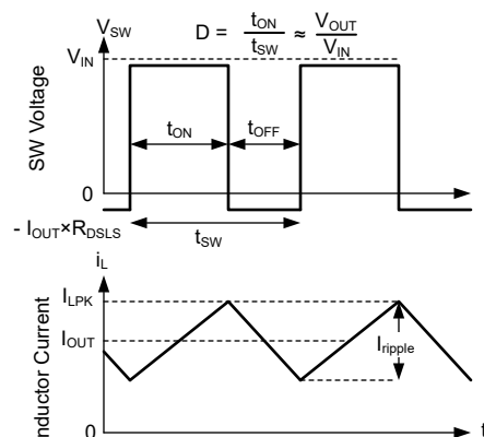
Figure 6-9. SW Voltage and Inductor Current Waveforms in Continuous Conduction Mode (CCM)
