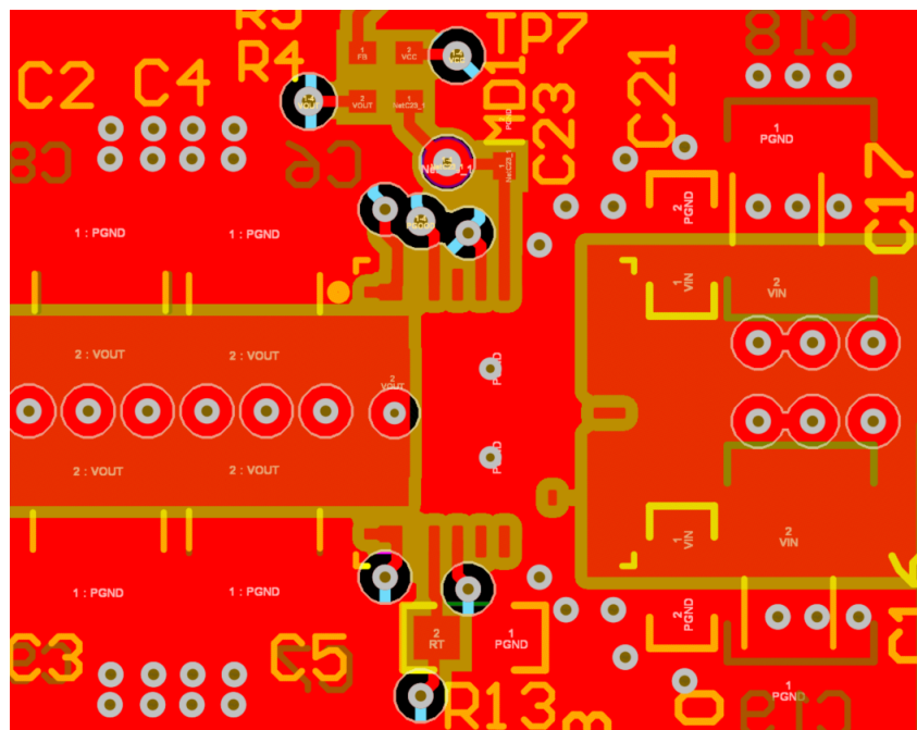
Figure 7-19. Layout Example
