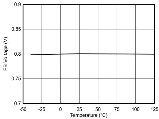
Figure 5-1. Feedback Voltage
