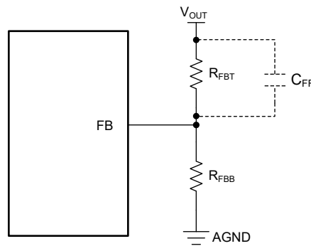
Figure 6-1. Setting Output Voltage of Adjustable Versions
