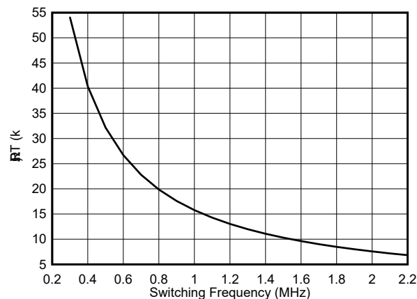
Figure 6-6. Switching Frequency vs RT
