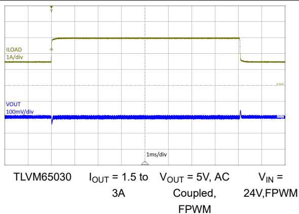
Figure 7-14. Load Transient (50 to 100%)
