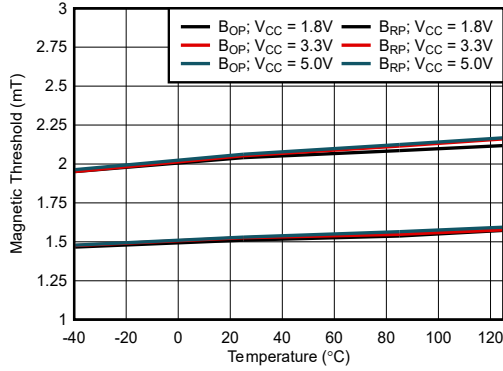
Figure 6-5. 2.0mT B OP and B RP Thresholds vs Temperature
