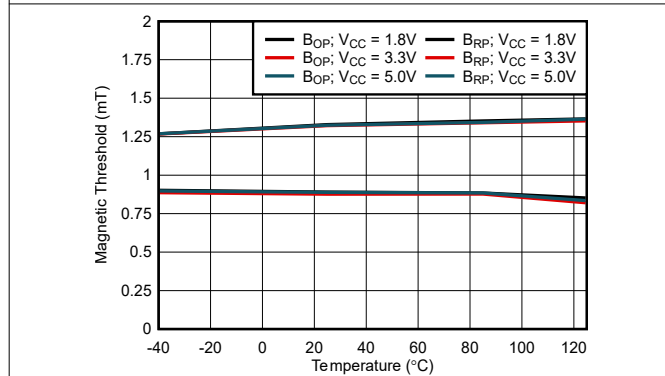
Figure 6-3. 1.3mT B_{OP} and B_{RP} Thresholds vs Temperature
