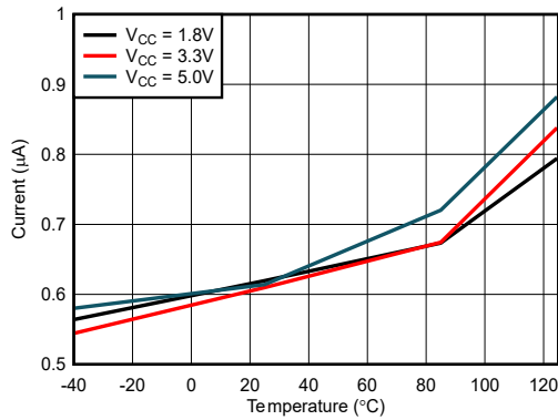
Figure 6-7. 5Hz I CCAVG vs Temperature
