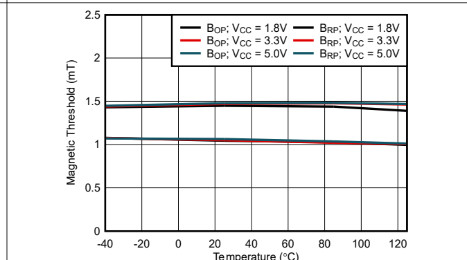
Figure 6-4. 1.5mT B_{OP} and B_{RP} Thresholds vs Temperature
