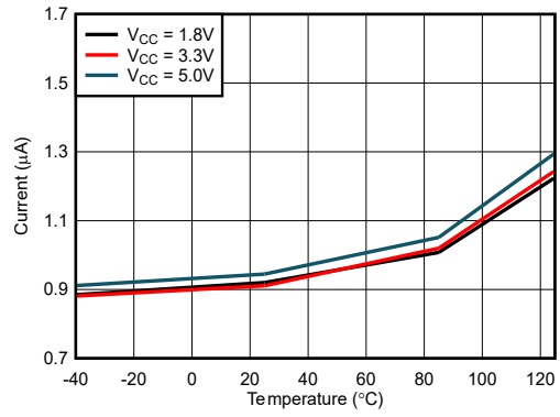
Figure 6-8. 10Hz I CCAVG vs Temperature
