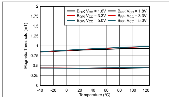
Figure 6-1. 0.9mT B_{OP} and B_{RP} Thresholds vs Temperature
