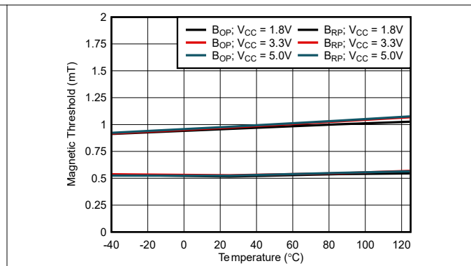
Figure 6-2. 1.0mT B_{OP} and B_{RP} Thresholds vs Temperature
