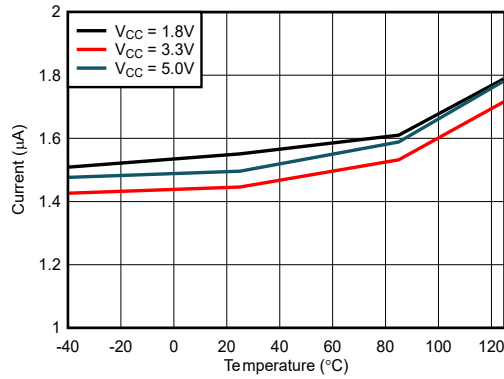
Figure 6-9. 20Hz I CCAVG vs Temperature
