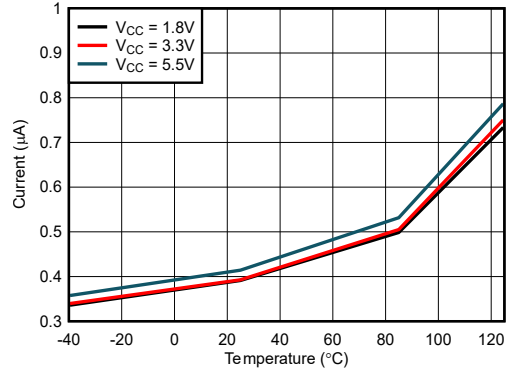
Figure 6-6. 1.25Hz I CCAVG vs Temperature
