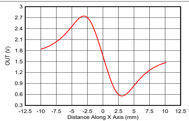
Figure 9-7. Output Voltage of TMAG5253B When The Magnet Slides by on Top of the Sensor
