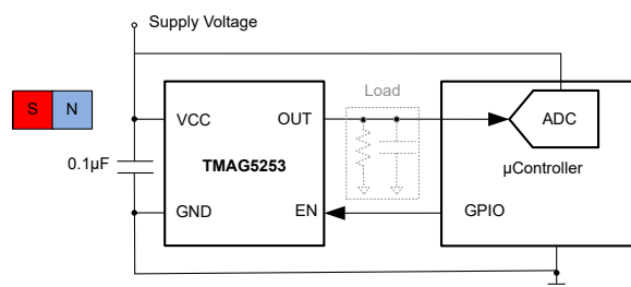
Typical Schematic
