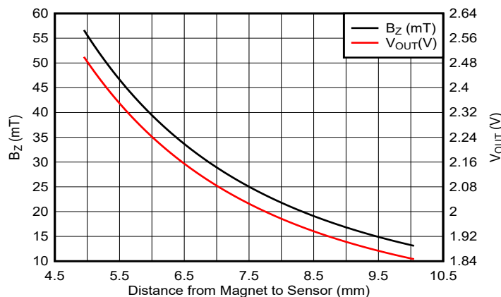
Figure 9-9. Magnetic Field ( B_z ) and the Output Voltage of the Sensor ( V_{OUT} ) vs the Distance from Magnet to the Sensor in TMAG5253B
