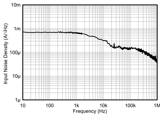
Figure 6-21. Input-Referred Noise Density vs Frequency
