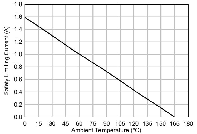
Figure 6-24. Thermal Derating Curve for Safety-Limiting Current, Side 2
