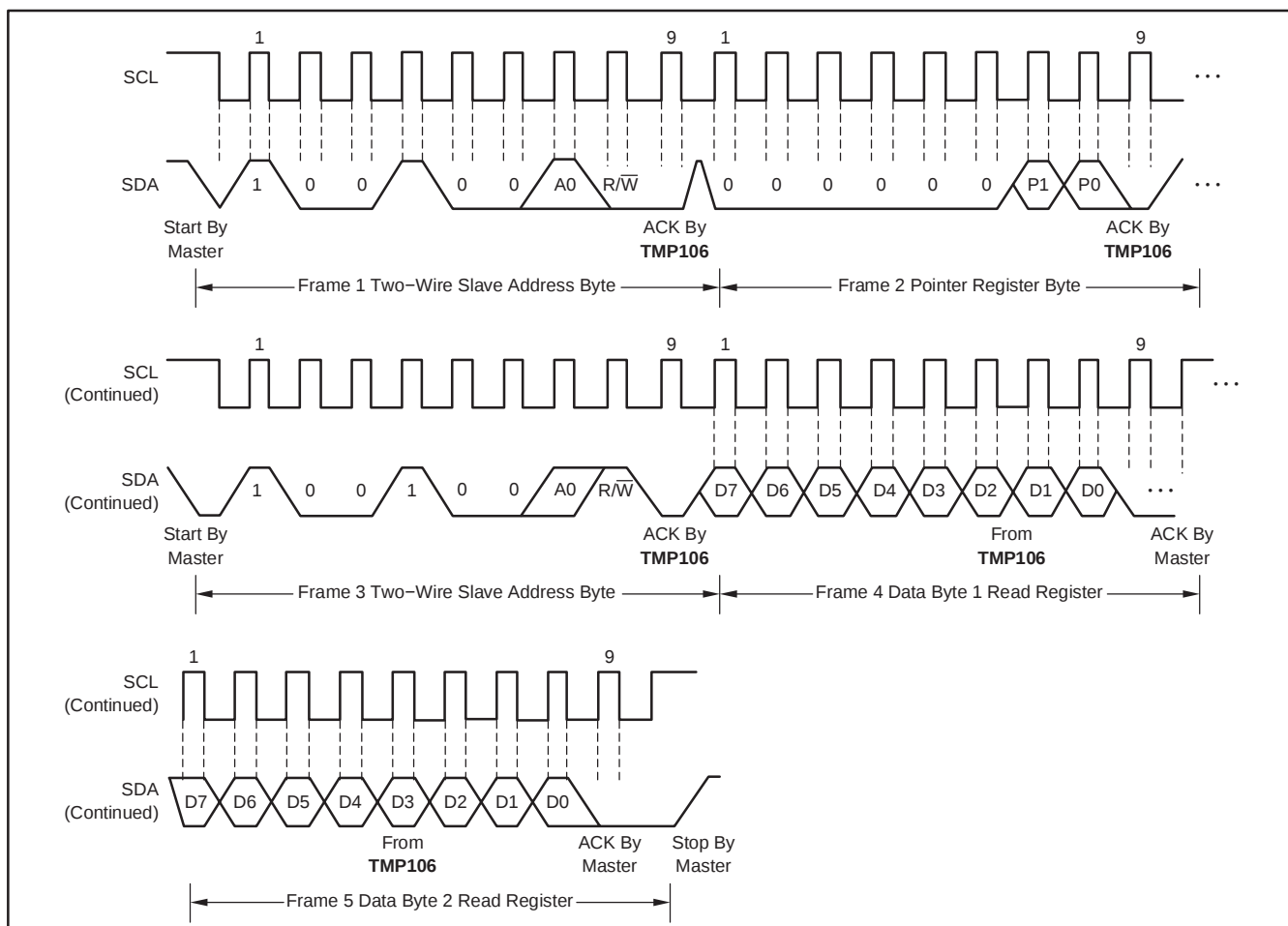
Figure 6. Two-Wire Timing Diagram for TMP106 Read Word Format
