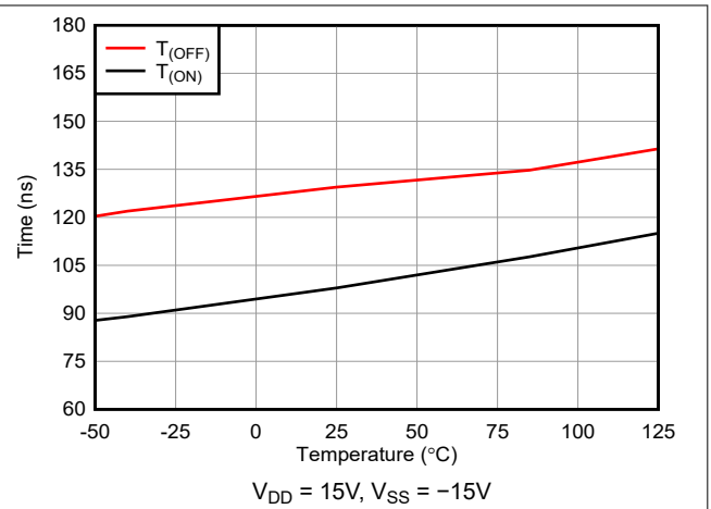
Figure 5-20. T_{\text{ON}} (EN) and T_{\text{OFF}} (EN) vs Temperature
