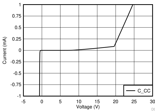
Figure 7-29. C CC IV Curve
