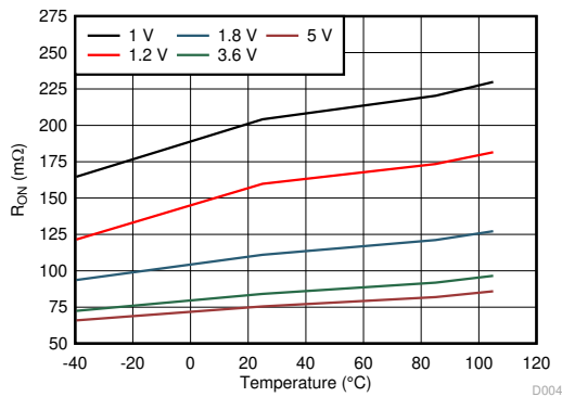
Figure 7-3. ON-Resistance ( R_{ON} )
