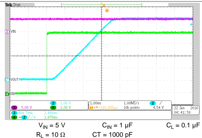
Figure 13. Rise Time ( t_R ) at V_{IN} = 5 V
