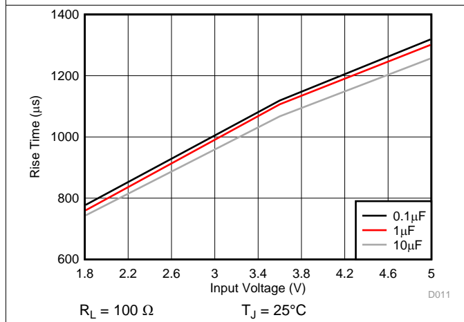
Figure 11. Rise Time vs Input Voltage Across Load Capacitance
