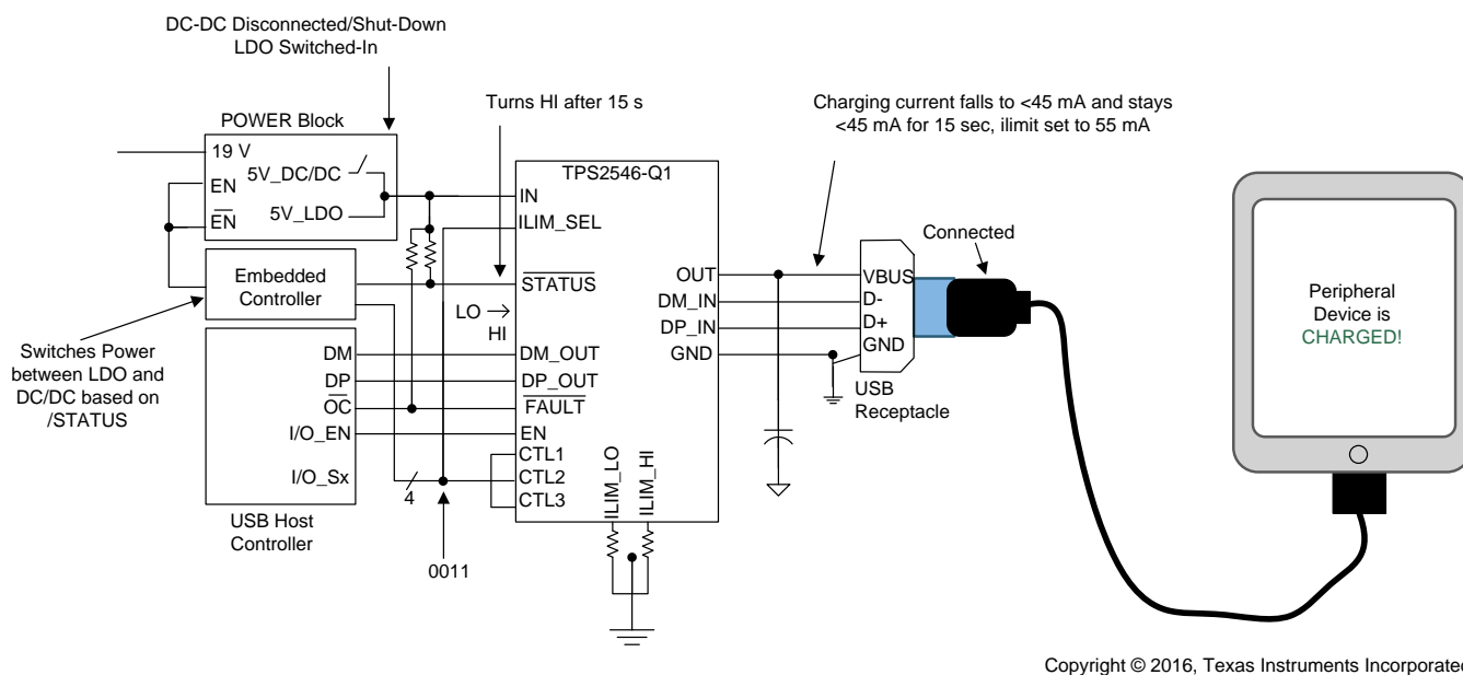
Figure 35. Case 2B: System in S4/S5, Attached Device Fully Charged
