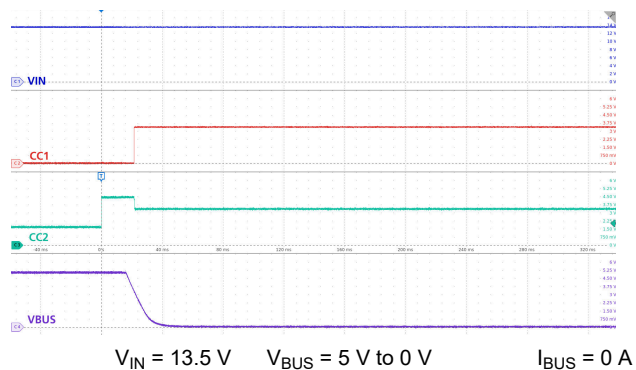
Figure 9-13. Type-C Detach
