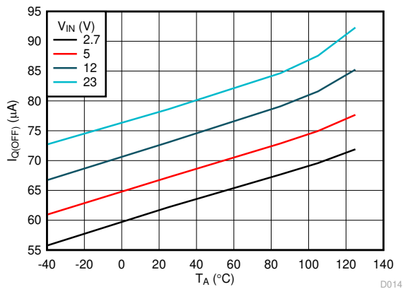
Figure 6-6. IN OFF State (UVLO) Current vs Temperature
