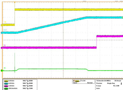
C_{OUT} = 220\mu F , C_{dVdt} = 10nF , EN/UVLO connected to IN through resistor ladder, 12V hot-plugged to IN
