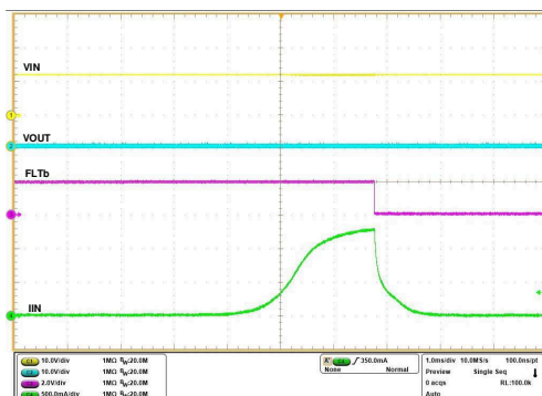
Figure 6-53. Output Short-Circuit During Steady State
