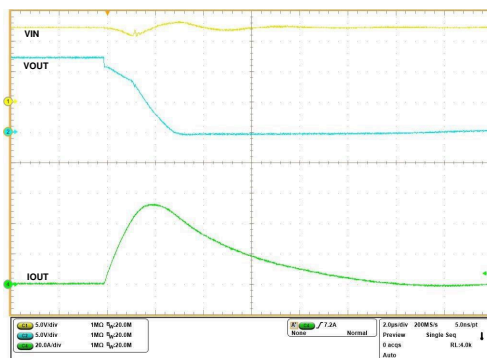
Figure 6-52. Circuit Breaker Response - TPS259474x
