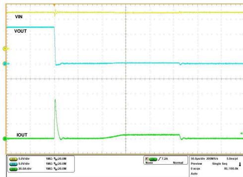
Figure 6-51. Transient Overcurrent Blanking Timer Response - TPS259474x
