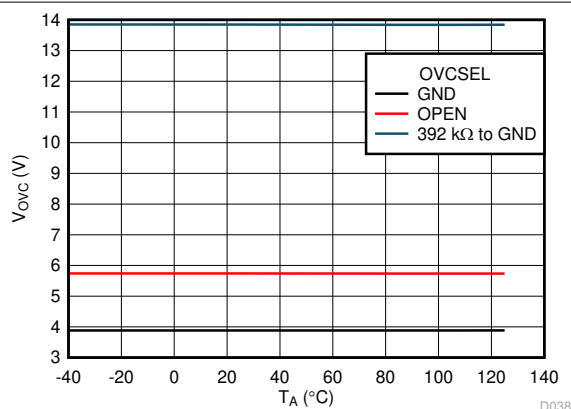
Figure 6-24. OVC Threshold vs Temperature
