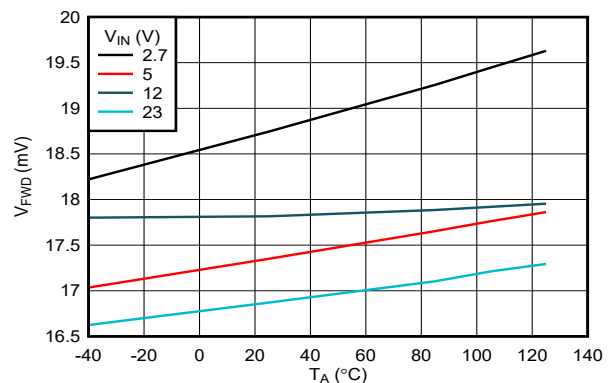
Figure 6-19. RCB - Forward Regulation Voltage vs Temperature
