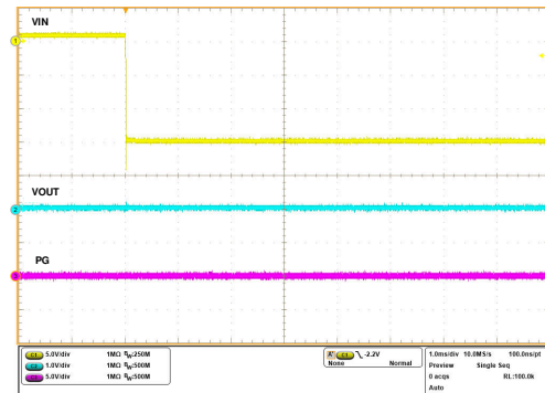
C_{OUT} = 220\mu F , PG pulled up to 3V, -15V hot-plugged to IN
