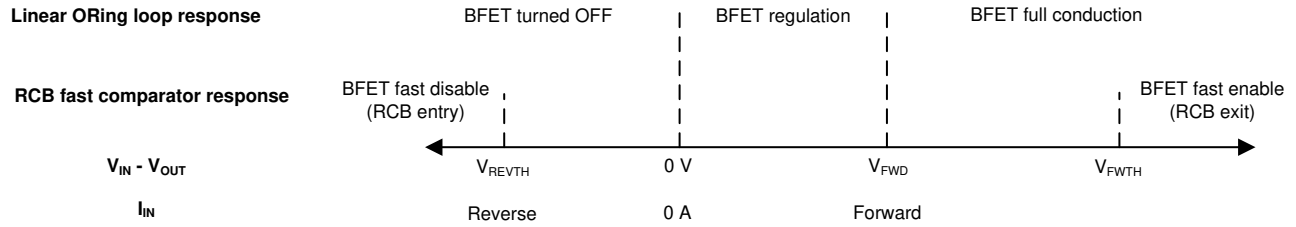
Figure 7-13. Reverse Current Blocking Response
