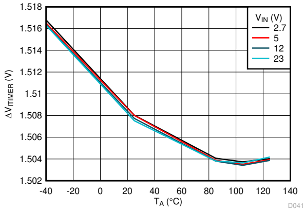
Figure 6-28. ITIMER Discharge Differential Voltage Threshold vs Temperature
