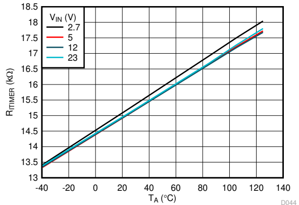
Figure 6-30. ITIMER Internal Pullup Resistance vs Temperature
