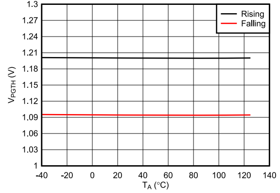
Figure 6-33. PGTH Threshold vs Temperature
