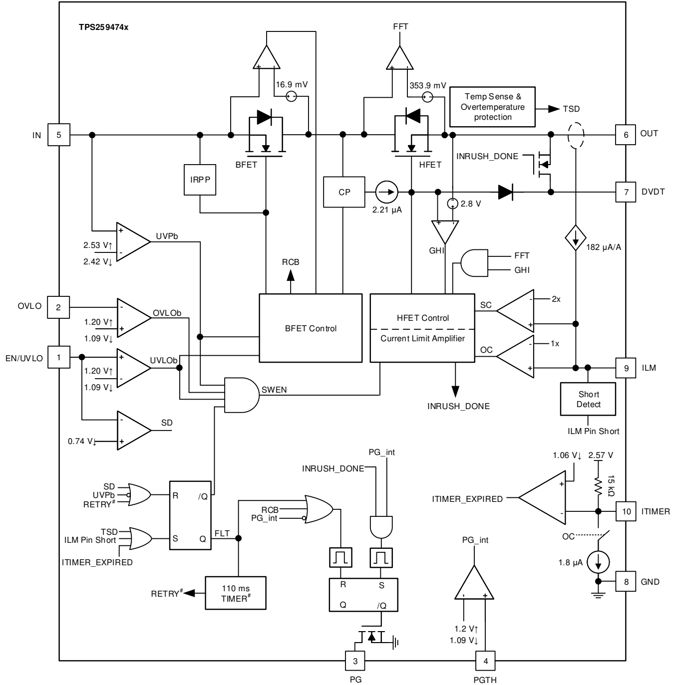
Figure 7-3. TPS25947x Block Diagram
