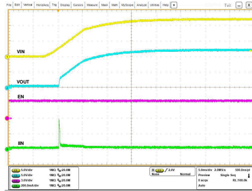
V_{EN/UVLO} = 3.3V , C_{OUT} = 30\mu F , C_{dVdt} = \text{Open} , V_{IN} ramped up to 12V
