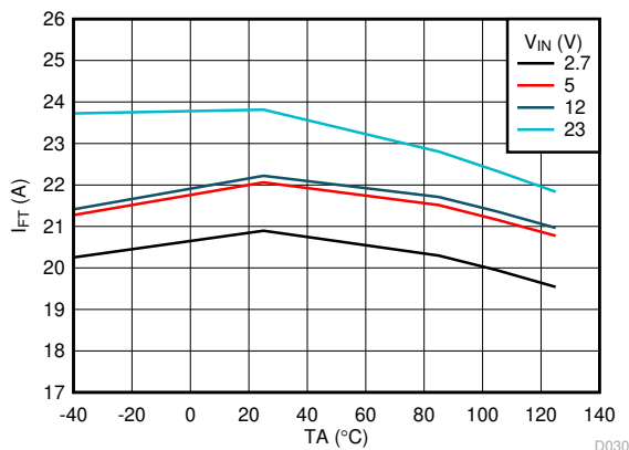
Figure 6-18. Steady State Fixed Fast-Trip Current Threshold vs Temperature
