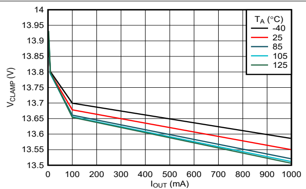
Figure 6-25. OVC Clamping Voltage (OVCSEL = 392kΩ to GND) vs Load Current
