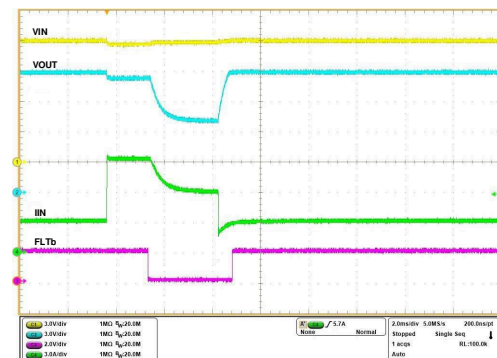
V_{IN} = 12\text{V} , C_{TIMER} = 2.2\text{nF} , C_{OUT} = 220\mu\text{F} , R_{ILM} = 549\Omega , I_{OUT} stepped from 3A → 9A → 3A within 5ms
