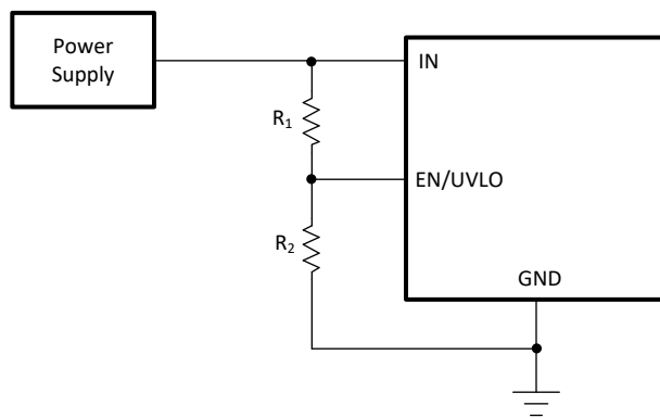
Figure 7-4. Adjustable Undervoltage Protection
