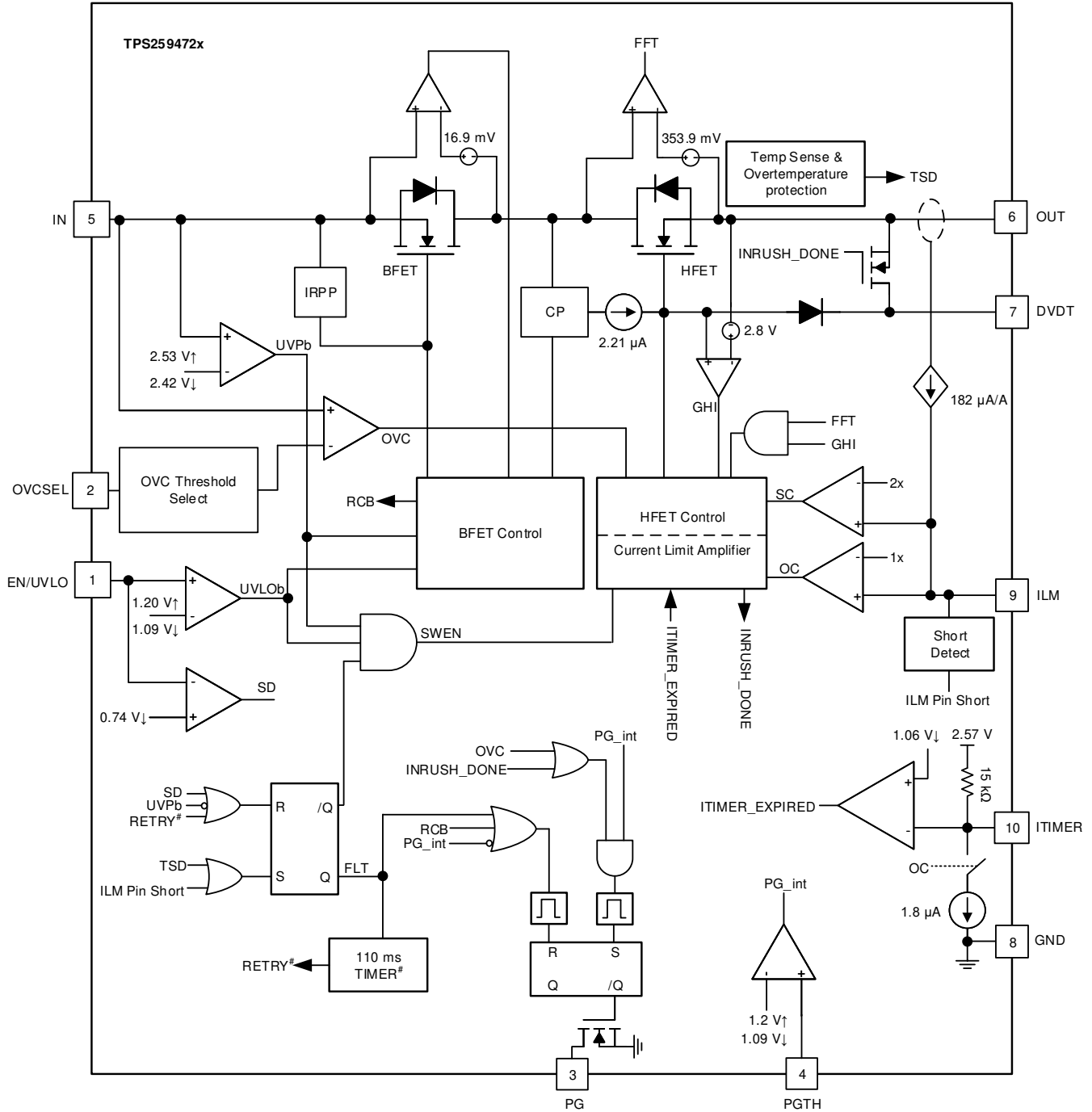
Figure 7-2. TPS259472x Block Diagram
