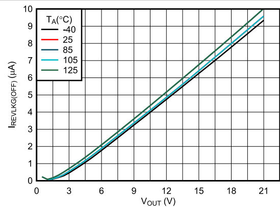
Figure 6-23. Reverse Leakage Current During OFF-State
