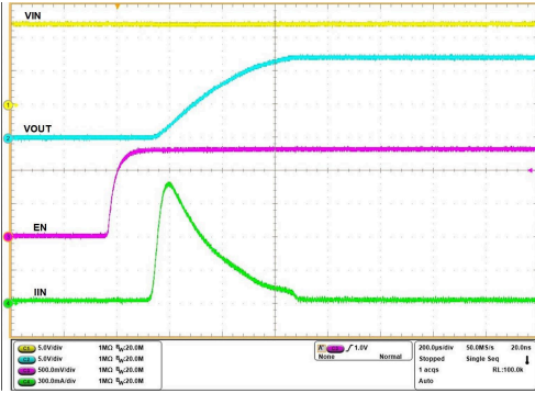
V_{IN} = 12V , C_{OUT} = 30\mu F , C_{dVdt} = \text{Open} , V_{EN/UVLO} stepped up to 1.4V
