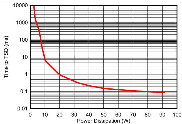
Figure 6-36. Time to Thermal Shut-Down During Inrush State
