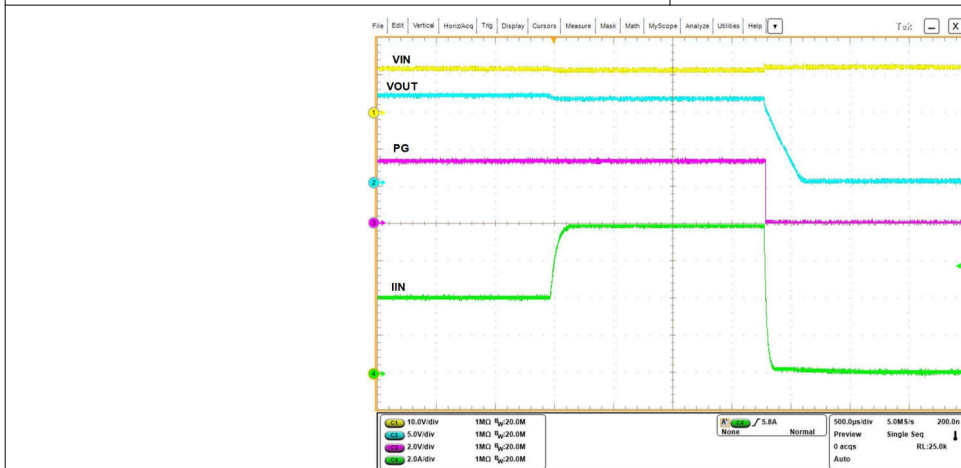
Figure 8-6. Circuit Breaker Response
