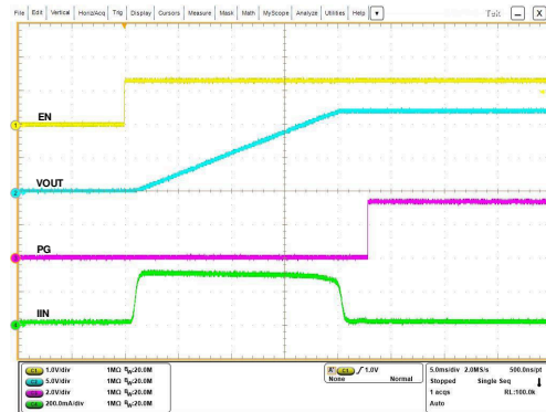
V_{IN} = 12V , C_{OUT} = 470\mu F , C_{dVdt} = 3300pF , V_{EN/UVLO} stepped up to 1.4V
