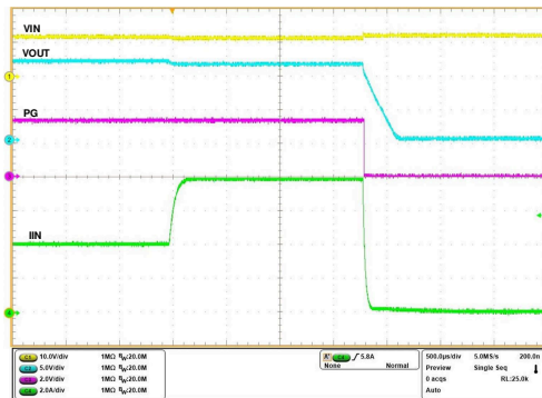
Figure 6-50. Active Current Limit Response Followed by TSD - TPS259470x
