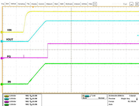
V_{IN} = 12V , C_{OUT} = 470\mu F , R_{OUT} = 5\Omega , C_{dVdt} = 3300pF , V_{EN/UVLO} stepped up to 1.4V
