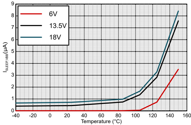
Figure 6-5. VBB Sleep Current ( I_{SLEEP,VBB} ) vs Temperature
