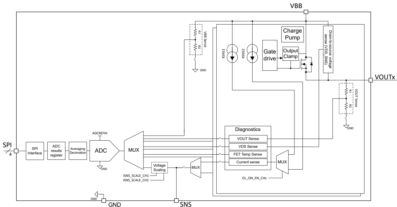
Figure 8-18. Integrated ADC Functional Block Diagram
