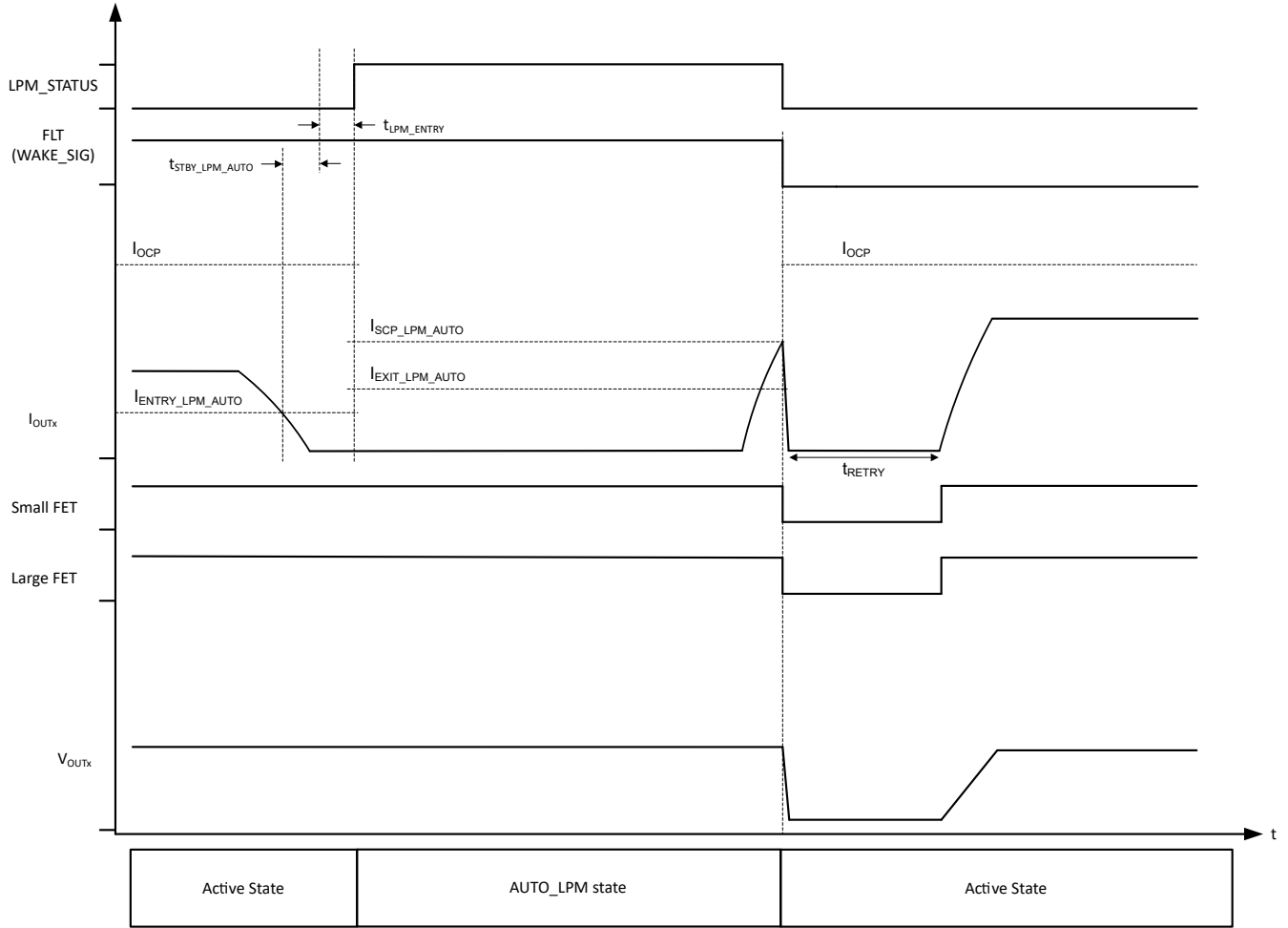
Figure 8-35. Load Increase Above I_{\text{SCP\_LPM\_AUTO}} and Below I_{\text{OCP}} in AUTO_LPM State
