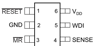
Figure 5-3. TPS3110 DBV Package 6-Pin SOT-23 Top View
