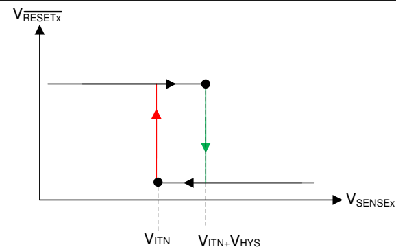
Figure 8-6. Hysteresis (Undervoltage Active-High)
