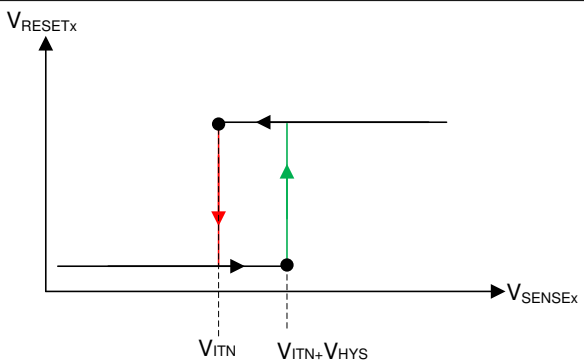
Figure 8-7. Hysteresis (Undervoltage Active-Low)
