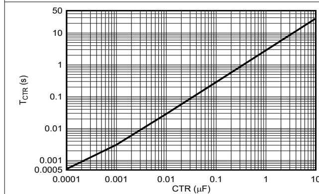
Figure 6-5. T_{CTR} vs CTR
