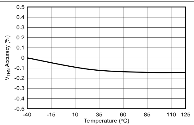
Figure 6-4. V_{THN} Accuracy vs Temperature
