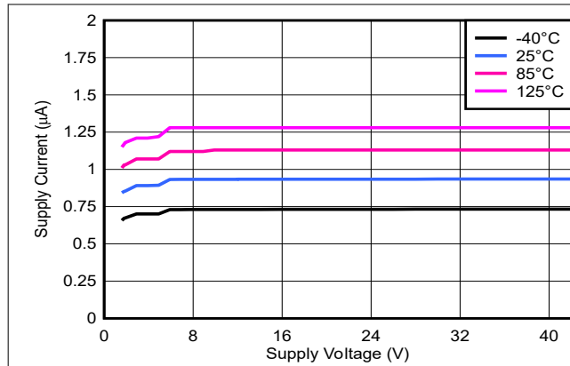
Figure 6-3. Supply Current vs Supply Voltage
