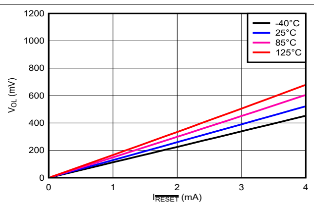
Figure 6-8. RESET Current (Sink) vs V_{OL} ( V_{DD} = 3.3\text{V} )
