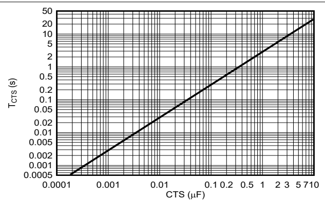
Figure 6-6. T_{CTS} vs CTS
