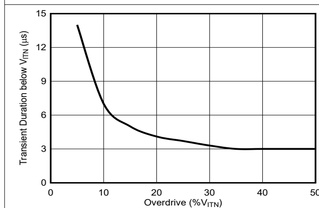
Figure 6-7. Transient Duration at Sense vs Sense Threshold Overdrive Voltage (CTS = Open)
