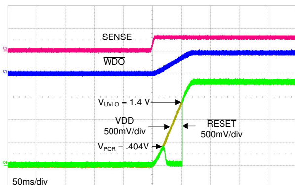
Figure 8-7. Startup Waveform
