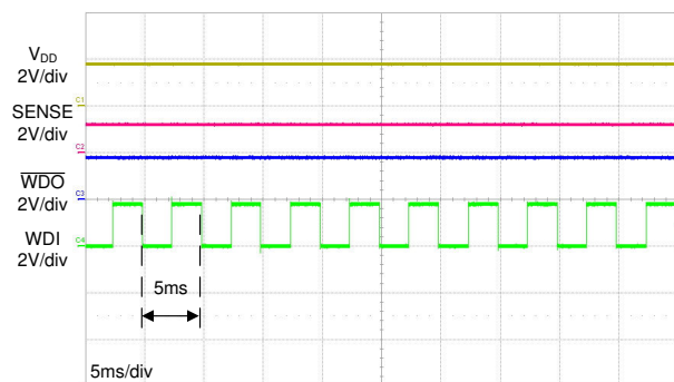
Figure 8-9. 200-Hz WDI Pulse
