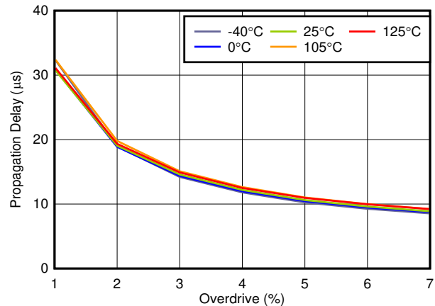
Figure 6-17. Propagation Delay vs Overdrive
