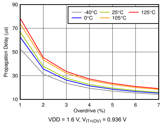
Figure 6-14. Propagation Delay vs Overdrive
