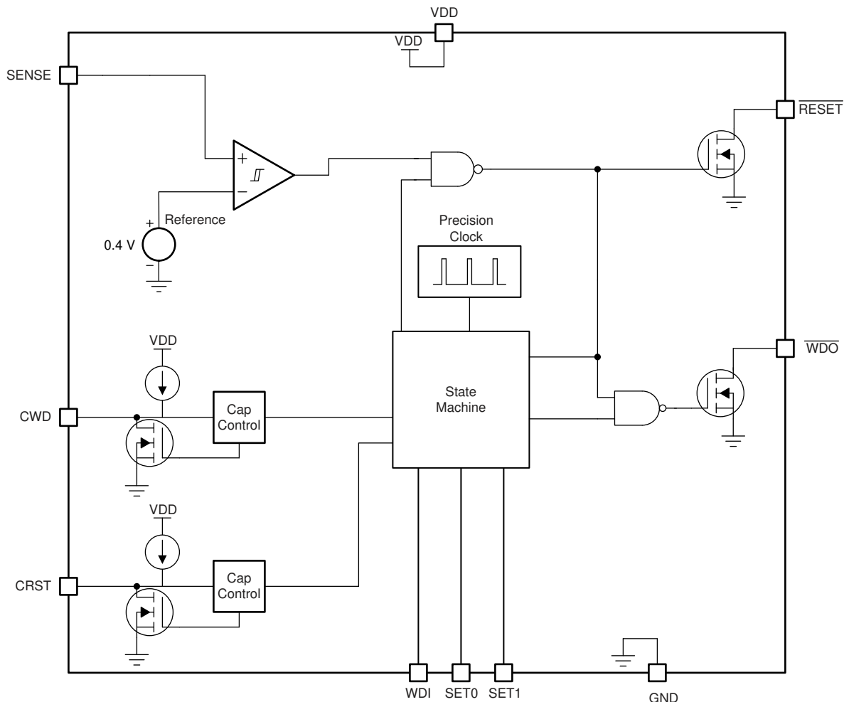
Figure 7-2. Adjustable Version Block Diagram
