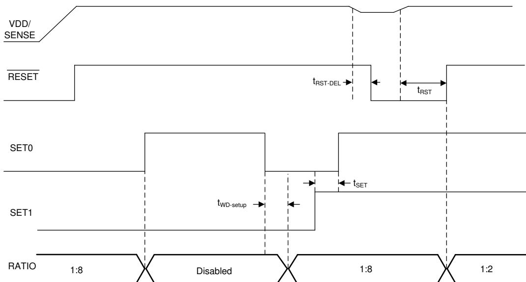
Figure 6-3. Changing SET0 and SET1 Pins
