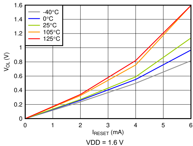
Figure 6-12. Low-Level \overline{\text{RESET}} Voltage vs \overline{\text{RESET}} Current
