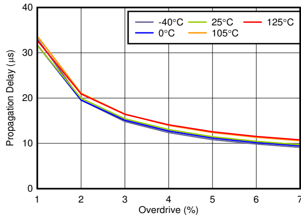
Figure 6-16. Propagation Delay vs Overdrive
