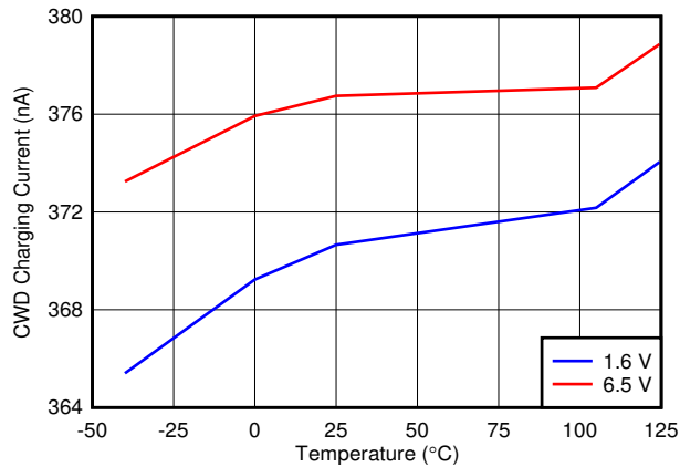
Figure 6-10. CWD Charging Current vs Temperature
