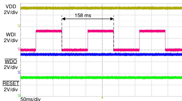
Figure 8-14. Typical WDI Signal
