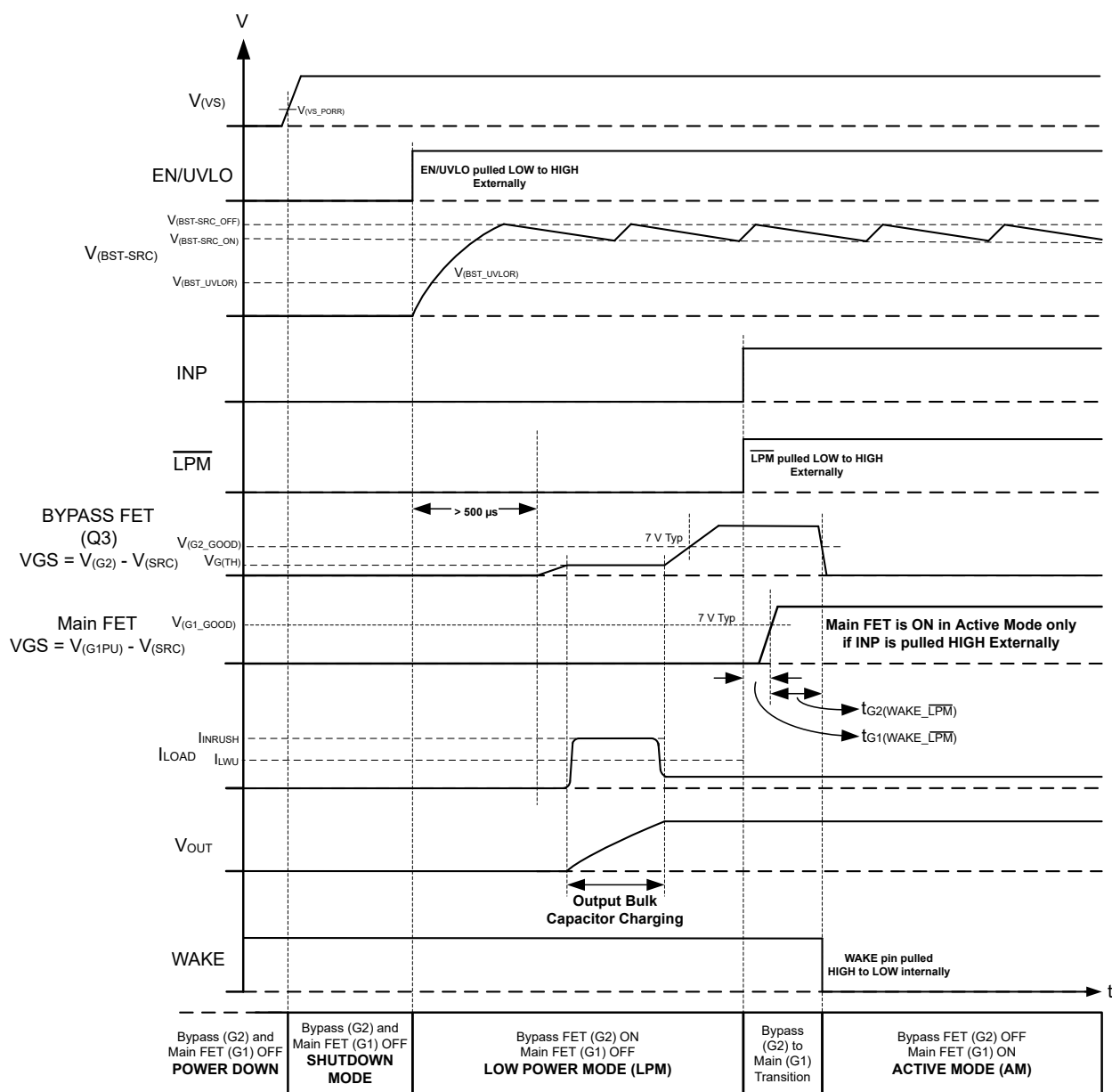
Figure 7-14. State Transition Timing Diagram With LPM Trigger
