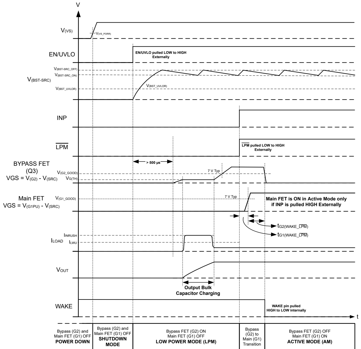
Figure 7-14. State Transition Timing Diagram With \overline{LPM} Trigger
